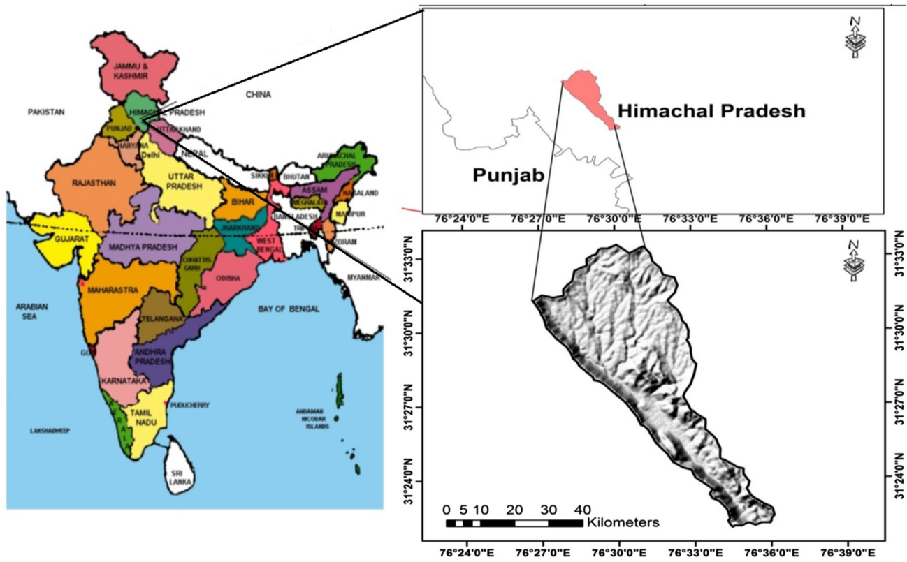
Fig. 1 Location map of the Sheer Khadd River basin
