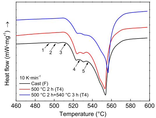
Fig. 2: DSC curves of Al-12Si-4Cu-2Ni-0.8Mg-0.2Gd alloy with different solution treatments
