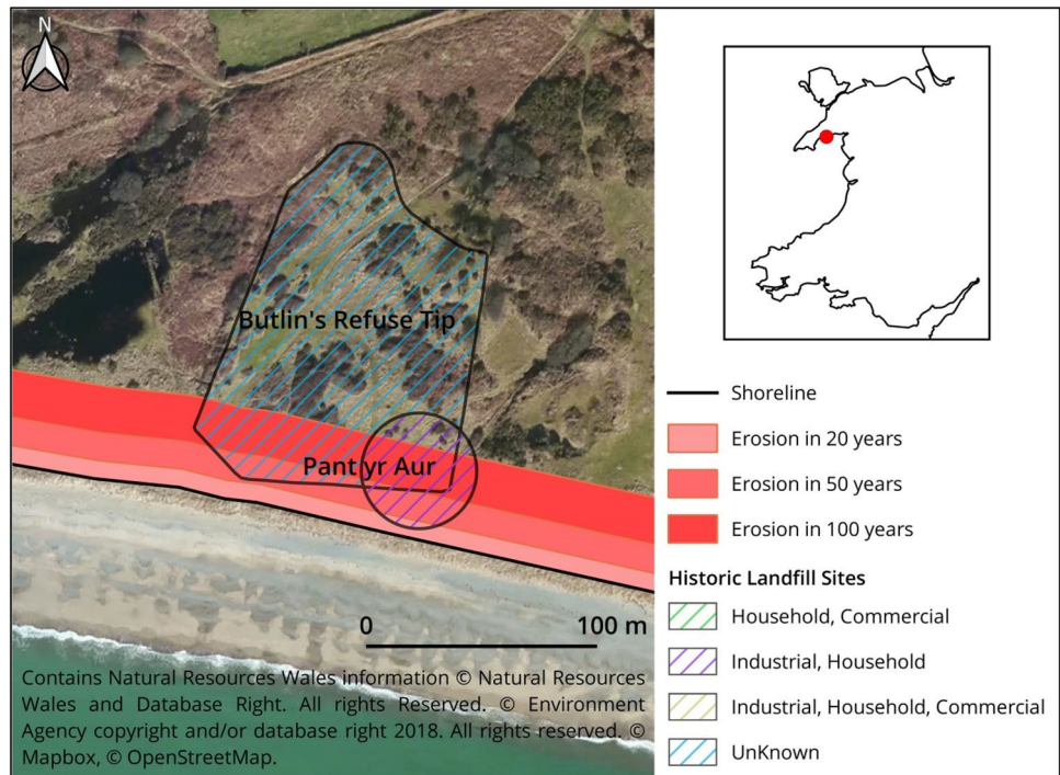
Fig. 6 Location of Butlin’s refuse tip and Pant-yr-Aur sites with predicted erosion buffers
