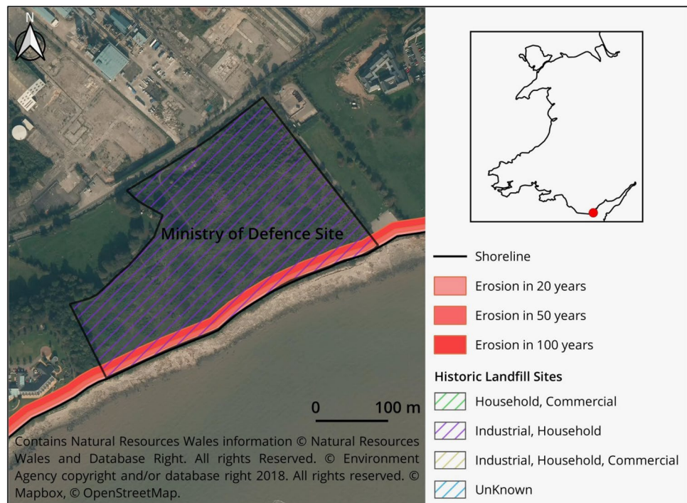
Fig. 3 Location of Ministry of Defence site with predicted erosion buffers
