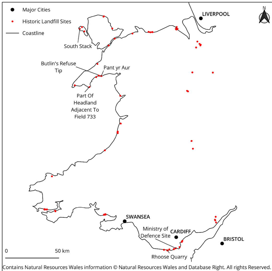
Fig. 1 Historic landfill sites location in Wales
