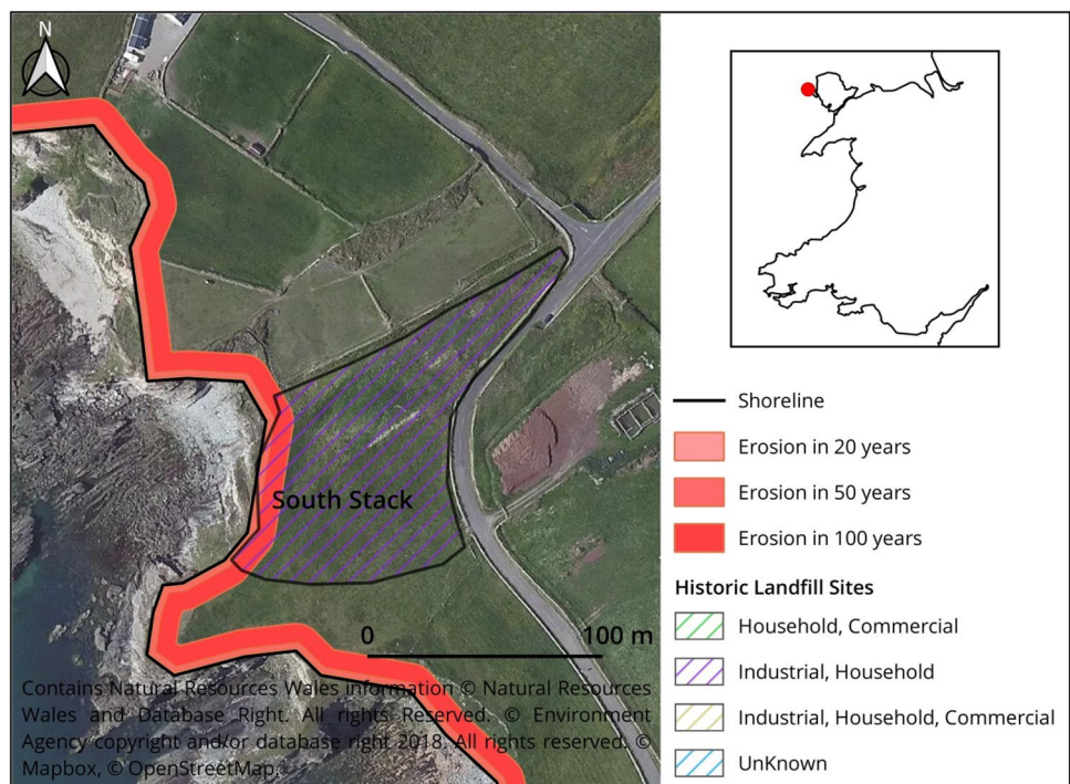
Fig. 7 Location of South Stack site with predicted erosion buffers
