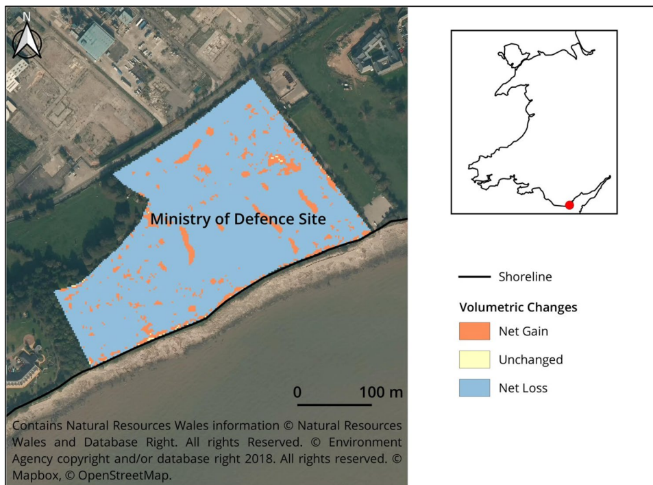
Fig. 4 Topsoil volumetric change (2006–2015) at Ministry of Defence landfill site
