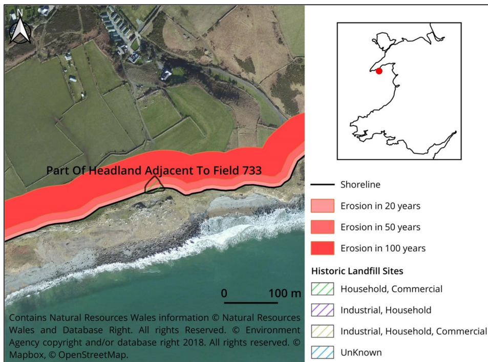
Fig. 5 Location of part of headland adjacent to field 733 site with predicted erosion buffers
