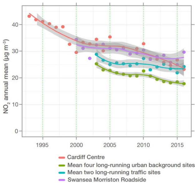
Fig. 2 Annual mean nitrogen dioxide (NO 2 ) concentration at long running sites in Wales (Adopted from Welsh Air Quality Forum (2017))
