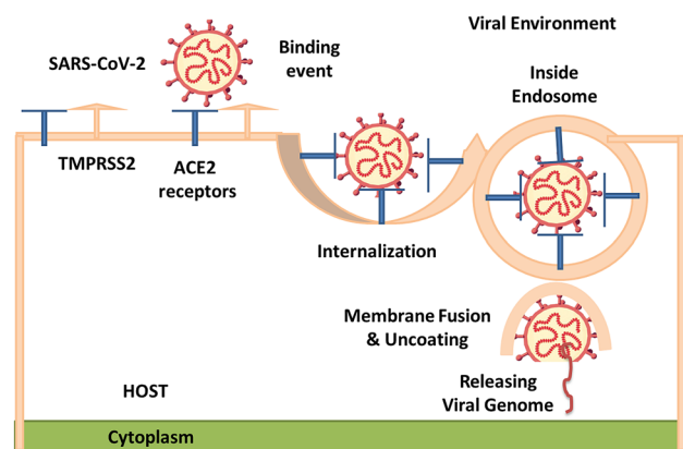
Fig. 2 Interaction of SARS-CoV-2 with host cell
