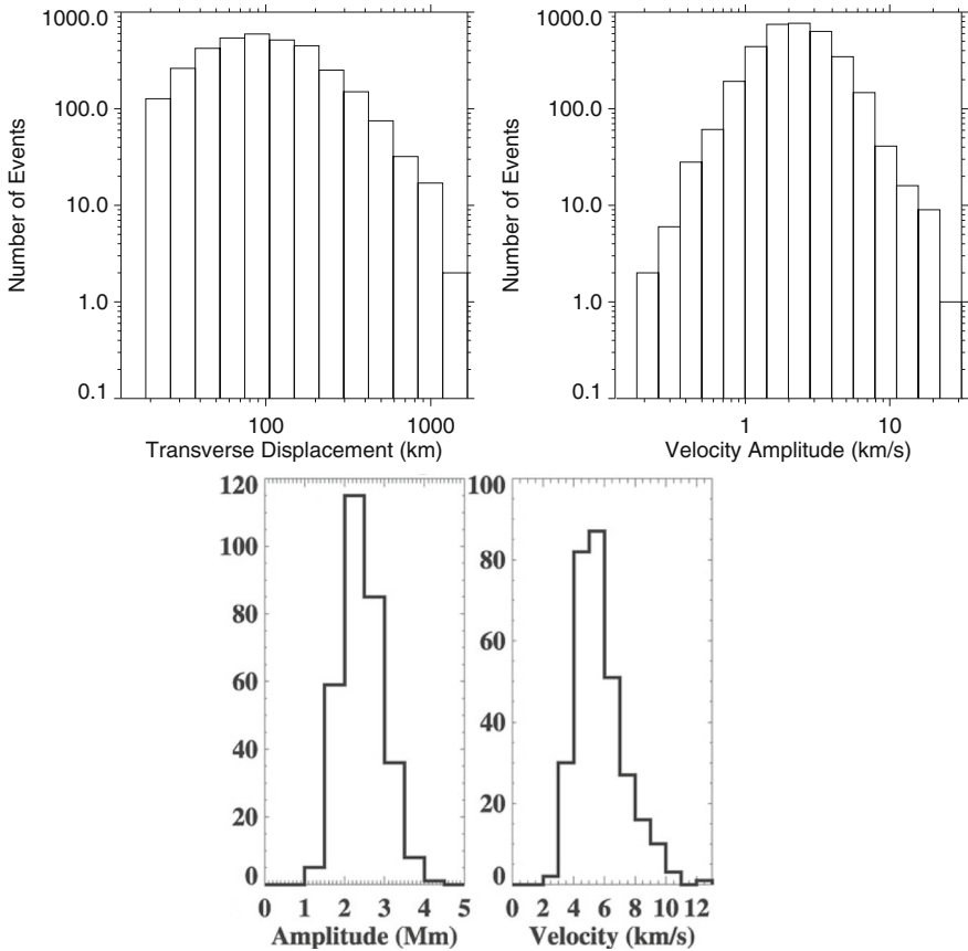
Fig. 12 Top: Hinode/SOT H_{\alpha} observation of transverse thread oscillations in a quiescent prominence. Image reproduced with permission from Hillier et al. (2013), copyright by AAS. Bottom: SDO/AIA 171 \text{\AA} observation of transverse oscillations of barb belonging to a polar crown prominence. Image reproduced with permission from Li and Zhang (2013), copyright by Springer. Histograms of (left) displacement amplitude and (right) velocity amplitude
