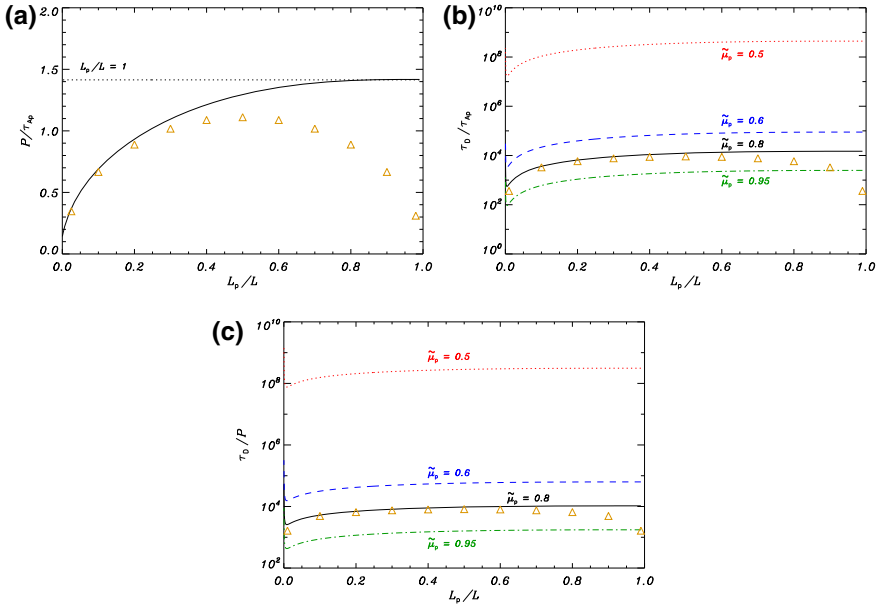
Fig. 80 Results for the thread model in Fig. 79 without transverse transitional layer and for the prominence thread located at the central part of the magnetic tube. a Period, P , of the fundamental kink mode in units of the internal Alfvén travel time, \tau_{Ap} , as a function of L_p/L . The horizontal dotted line corresponds to the period of the kink mode in a homogeneous prominence cylinder. The symbols are the analytic solution (Eq. 24 in Soler et al. 2010a). b Damping time, \tau_d , in units of the internal Alfvén travel time, \tau_{Ap} , as a function of L_p/L . The different lines denote \tilde{\mu}_p = 0.5 (dotted), 0.6 (dashed), 0.8 (solid) and 0.95 (dash-dotted). The symbols are the analytic approximation for \tilde{\mu}_p = 0.8 (Eq. 27 in Soler et al. 2010a). c \tau_d/P versus L_p/L . The line styles have the same meaning as in (b) and the symbols are the approximation given by Eq. (41). Image reproduced with permission from Soler et al. (2010a), copyright by AAS
