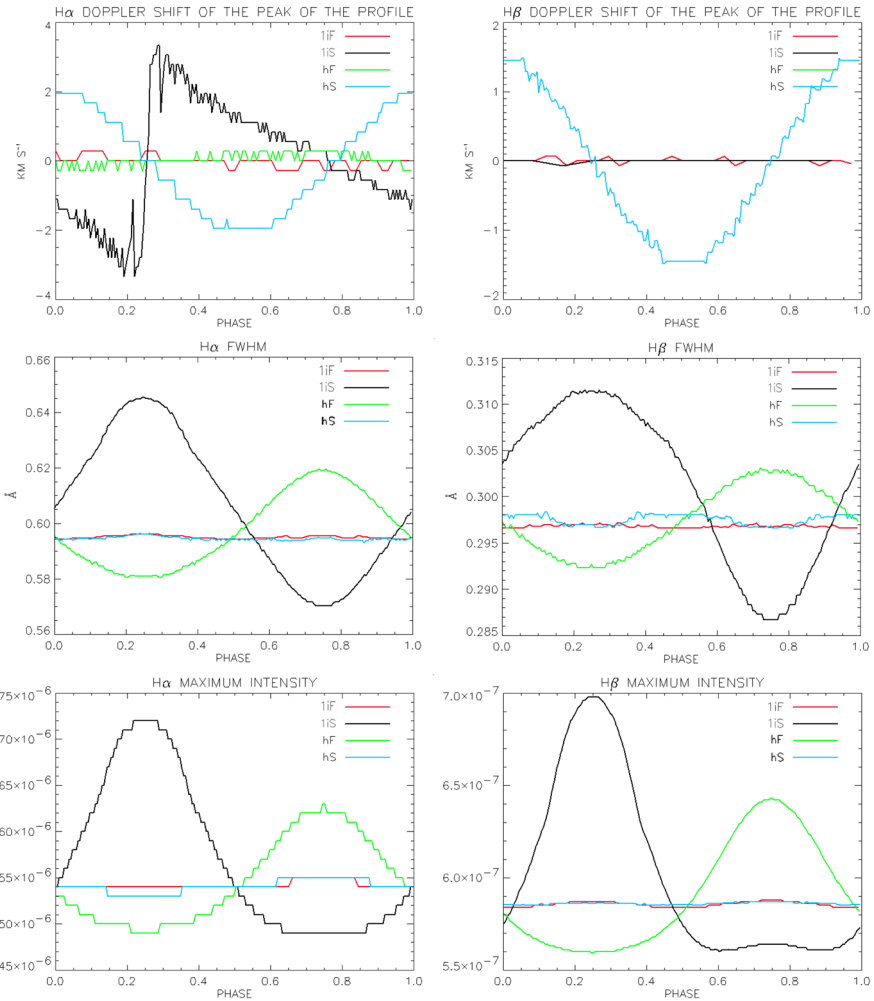
Fig. 62 MHD plus radiative transfer model: temporal variation of the spectral line parameters of the H_{\alpha} (left) and H_{\beta} (right) lines for the magnetoacoustic hS, hF, 1iS and 1iF modes (see text for an explanation of these acronyms). From top to bottom: Doppler velocity, full width at half maximum (FWHM) and line intensity. Image reproduced with permission from Zapiór et al. (2016), copyright by AAS
