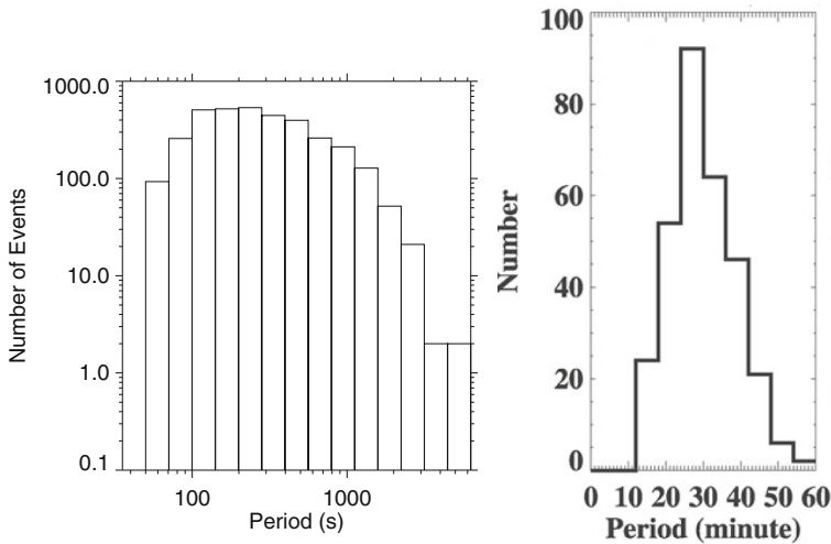
Fig. 9 Left: Hinode/SOT H\alpha observation of transverse thread oscillations in a quiescent prominence. Histogram of the initial period, P_0 of Eq. (8). Image reproduced with permission from Hillier et al. (2013), copyright by AAS. Right: SDO/AIA 171 Å observation of transverse oscillations of barbs belonging to a polar crown prominence. Histogram of the period. Image reproduced with permission from Li and Zhang (2013), copyright by Springer
