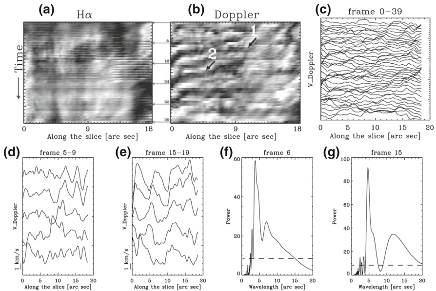
Fig. 32 a, b Time-slice diagrams of the H\alpha line intensity and Doppler shift along a filament thread. c Data of b shown as a set of curves instead of as a contour plot. Each curve represents the Doppler velocity along the thread for a fixed time (frame). d, e Signals from c for some selected times (frames). f, g Power spectrum of the Doppler shift along the thread for two times. Large peaks help identify the wavelength of propagating oscillations. Image reproduced with permission from Lin et al. (2007), copyright by Springer
