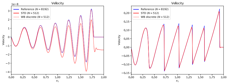
Fig. 11 Plot of the velocity profile for the small (left) and large (right) amplitude waves propagating up the isentropic atmosphere. The solid/dashed red lines are the solutions obtained with the standard/well-balanced scheme with N = 512 , respectively. In solid blue is also shown a reference solution obtained with the well-balanced scheme and N = 8192
