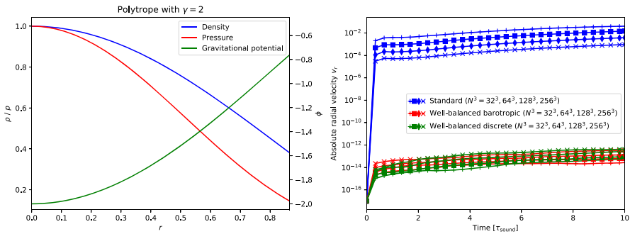
Fig. 13 Left panel: Radial density, pressure and gravitational potential profile of the polytrope up to the corners of the three-dimensional domain ( r = \sqrt{3}/2 \approx 0.87 ). Right panel: Maximum absolute radial velocity as a function of time in the simulations of the three-dimensional hydrostatic polytrope for the standard unbalanced/barotropic/discrete well-balanced second-order finite volume schemes
