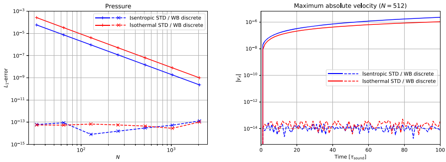
Fig. 9 Left panel: L_1 -norm of the difference between the initial and final pressure for the isentropic (solid and dashed blue lines) and isothermal (solid and dashed red lines) atmospheres after two sound crossing times for several resolutions. The solid and dashed lines represent the simulation performed with the standard and the well-balanced (WB) schemes, respectively. Right panel: The maximum absolute velocity as a function of time for N = 512
