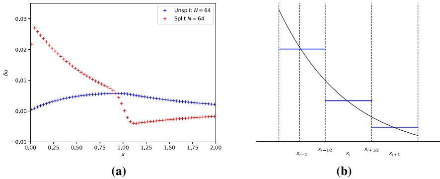
Fig. 3 The left panel shows the equilibrium perturbation for the numerically evolved steady state with a resolution of N = 64 cells at final time t_f = 1 . The blue and red pluses are obtained with the unsplit/split first-order schemes. The right panel shows the steady-state profile (solid black line) together with the cell averages \bar{U}_i^n (blue solid lines) at initial time for a few cells. The latter also corresponds to the piecewise constant reconstruction on which the unsplit/split first-order schemes are based
