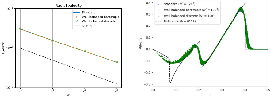
Fig. 15 Large perturbation on a three-dimensional polytrope. Left panel: L_1 -error of the radial velocity as a function resolution for the standard unbalanced, barotropic and discrete well-balanced second-order finite volume schemes. Right panel: Radial velocity scatter plot as a function of radius
