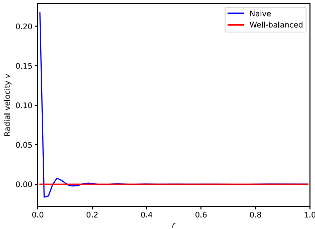
Fig. 6 The figure shows the radial velocity after one time unit of a constant state with unit density and pressure ( \rho = p = 1 ). The blue/red line corresponds to the results obtained by the standard naive/well-balanced second-order schemes from Sect. 2.5 with a resolution of N = 64 . In both simulations, solid wall boundary conditions were enforced at the upper boundary. From the plot it is obvious that the standard treatment of the geometric source term results in spurious velocity fluctuations near the origin. In contrast, the well-balanced scheme shows a still standing radial profile, as is expected
