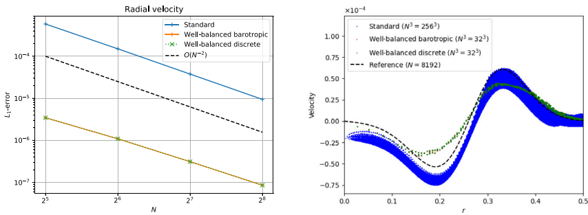
Fig. 14 Small perturbation on a three-dimensional polytrope. Left panel: L_1 -error of the radial velocity as a function resolution for the standard unbalanced, barotropic and discrete well-balanced second-order finite volume schemes. Right panel: Radial velocity scatter plot as a function of radius
