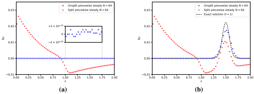
Fig. 4 The left panel shows the equilibrium perturbation for the numerically evolved steady state with a resolution of N = 64 cells at final time t_f = 1 . The blue and red pluses are obtained with the unsplit/split first-order schemes using the piecewise steady reconstruction. The zoom in shows that the unsplit scheme is able to preserve the steady state down to machine precision. The right panel shows the equilibrium perturbation for the slightly perturbed steady-state concentration simulated with the unsplit/split first-order schemes using the piecewise steady reconstruction. The unsplit scheme clearly relaxes back to the steady state away from the concentration perturbation
