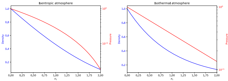
Fig. 8 Density and pressure profiles for the isentropic (left panel) and isothermal (right panel) atmospheres
