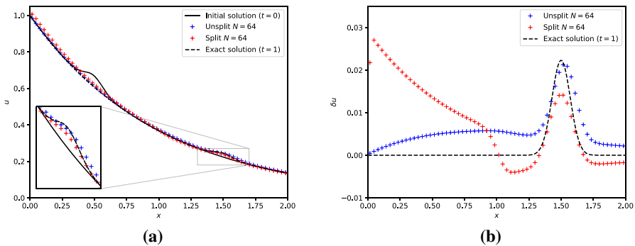
Fig. 2 The left panel shows the slightly perturbed steady state initial concentration Eq. (32) (solid black line) and the exact solution at the time final t_f = 1 (dashed black line). The same panel also shows the results obtained with the unsplit/split first-order schemes with a resolution of N = 64 cells. The right panel shows the equilibrium perturbation (solution minus the steady-state background) at the final time
