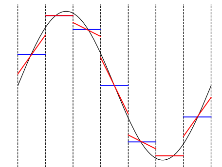
Fig. 1 Illustration of the reconstruction procedure for the sine function u(x) = \sin(x) (solid black line). Within each control volume or cell is shown the cell average \bar{U}_i (solid blue) and a piecewise linear TVD/MUSCL reconstruction U_i(x) (solid red). Notice the limiter’s action near the two extrema, where the slopes are clipped to ensure the monotonicity of the reconstruction. The piecewise constant cell averages correspond to a piecewise constant reconstruction
