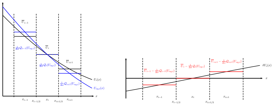
Fig. 5 Sketch of the piecewise steady reconstruction of some scalar quantity from the cell averages \{\bar{U}_k\} . For the illustration, we assume that the steady-state projection of the cell averages is trivial \bar{U}_{eq,i} = \bar{U}_i as for the steady states of the linear advection–reaction equation. Left panel: At the beginning of the reconstruction process, we are given the cell averages of the i -th cell and its immediate neighbors (solid black piecewise constant lines). The equilibrium reconstruction U_{eq,i}(x) is built such that it matches the cell average \bar{U}_i by Eq. (47) and extrapolated to the neighboring cells k = i \pm 1 (solid blue line). The cell averages of U_{eq,i}(x) are then computed in the neighboring cells k = i \pm 1 (solid blue piecewise constant lines) and the cell-averaged equilibrium perturbations as seen from the i -th cell are computed. Right panel: The equilibrium perturbation \delta U_i(x) is reconstructed by a standard reconstruction procedure Eq. (48). Finally, by combining the equilibrium U_{eq,i}(x) and perturbation \delta U_i(x) reconstruction as Eq. (46) one obtains the equilibrium-preserving piecewise steady reconstruction U_i(x) in the left panel (solid black line)
