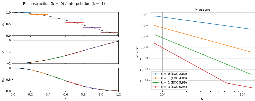
Fig. 7 Equilibrium pressure profile for a polytrope of index n = 1 ( \gamma = 2 ) over the radial interval [0, 1.2] discretized by 6 cells: Examples for the equilibrium density reconstruction \rho_{eq,i}(x) (based on the symmetric stencil \{\bar{\rho}_{-k}, \dots, \bar{\rho}_{+k}\} of size 2k + 1 ) and gravitational potential interpolation \phi_i(x) (based on the symmetric stencil \{\phi_{-k-1}, \dots, \phi_{+k+1}\} of the size 2k + 3 ) for the construction of the hydrostatic pressure profile p_{eq,i}(x) from Eq. (209). The left panel displays the equilibrium density as reconstructed with piecewise constants ( k = 0 ), the gravitational potential as interpolated with piecewise parabolic ( k = 1 ) and the resulting piecewise linear equilibrium pressure profile. The right panel shows the accuracy of the equilibrium pressure profile for several stencil size choices ( k = 0, 1, 2, 3 ) together with the estimated order of convergence (EOC). We empirically observe that the equilibrium pressure profile has accuracy \epsilon = 2(k + 1) , which is increased by one than one would have expected from the order of the equilibrium density reconstruction. We (presumably) attribute this increase in accuracy to a similar phenomena appearing in numerical integration, where even-degree (i.e., symmetric) Newton–Cotes quadrature rules have a by one higher order of accuracy than expected
