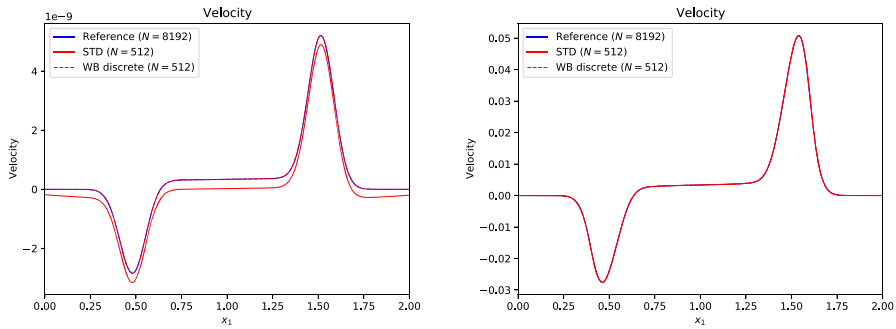
Fig. 12 Plot of the velocity profile for the small (left) and large (right) amplitude pressure perturbations on the isothermal atmosphere. The solid/dashed red lines are the solutions obtained with the standard/well-balanced scheme with N = 512 , respectively. In solid blue is also shown a reference solution obtained with the well-balanced scheme and N = 8192
