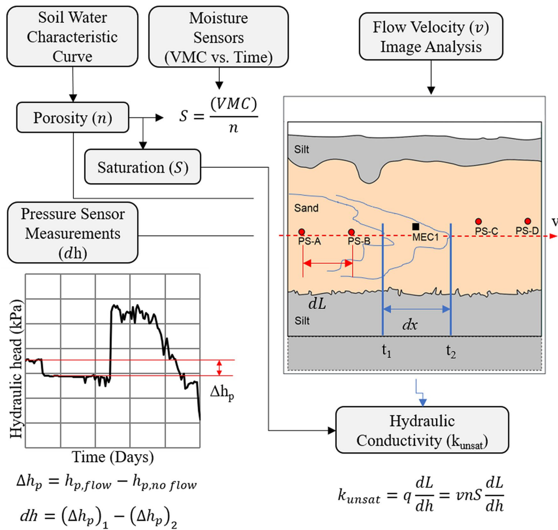
Fig. 8 Process for determining unsaturated permeability, through combination of various measurements
