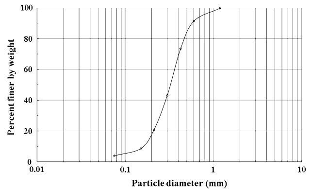
Fig. 2 Particle-size distribution of the soil
