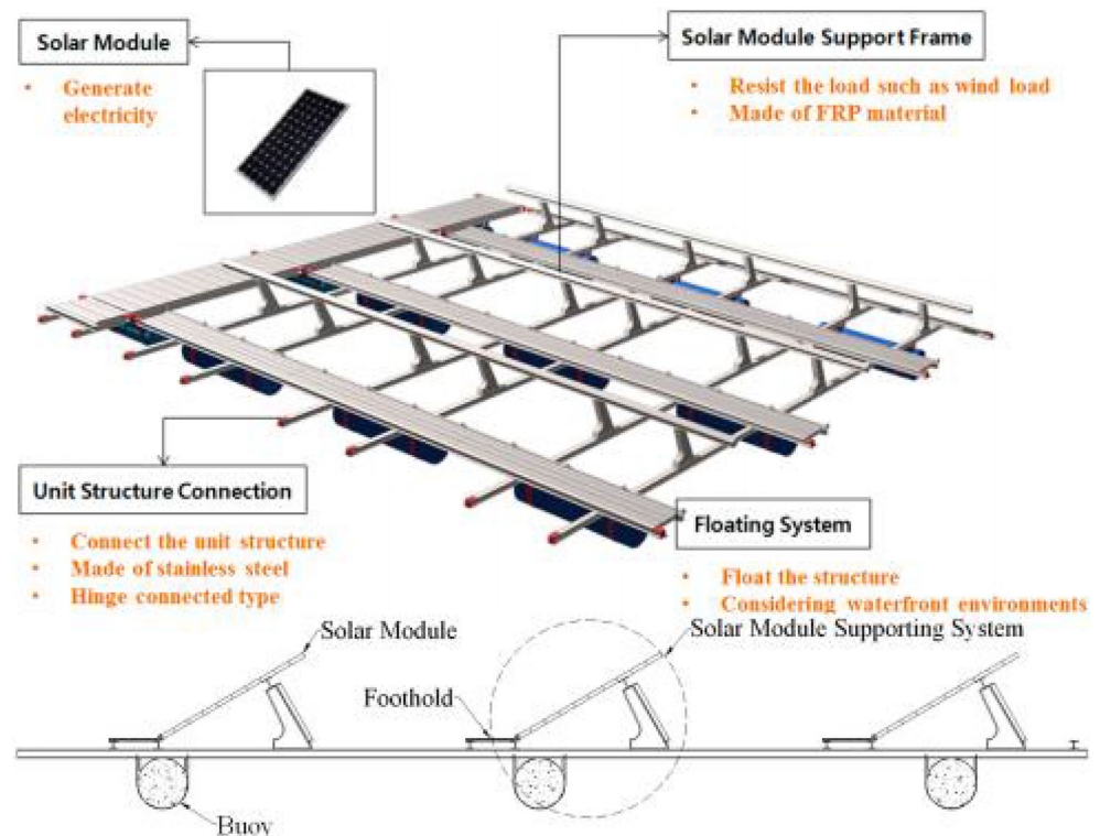
Fig. 4 Floating PV supporting structure
