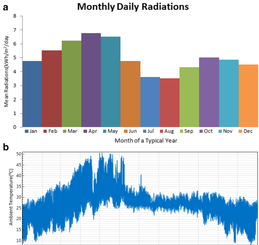
Fig. 1 a Month wise average daily radiations. b Ambient Temperature profile at selected project location
