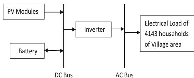
Fig. 3 PV system configuration
