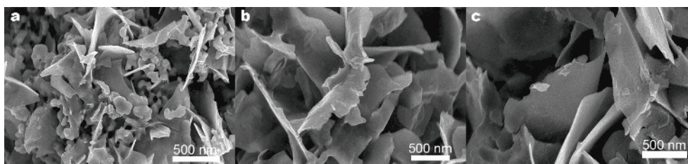
Figure S2 SEM images of as-prepared WN nanostructures at different hydrothermal pH values: (a) pH 0.5, (b) pH 1.5, and (c) pH 2.
