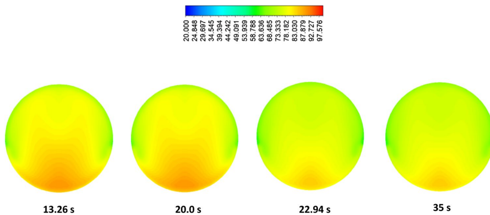
Fig. 10 Contours of temperature at plane P1 (catalyst inlet) for the case SS2 to SS1. The time instances of the contours are shown below each contour. The colorbar shows the temperature values in degrees Celsius
