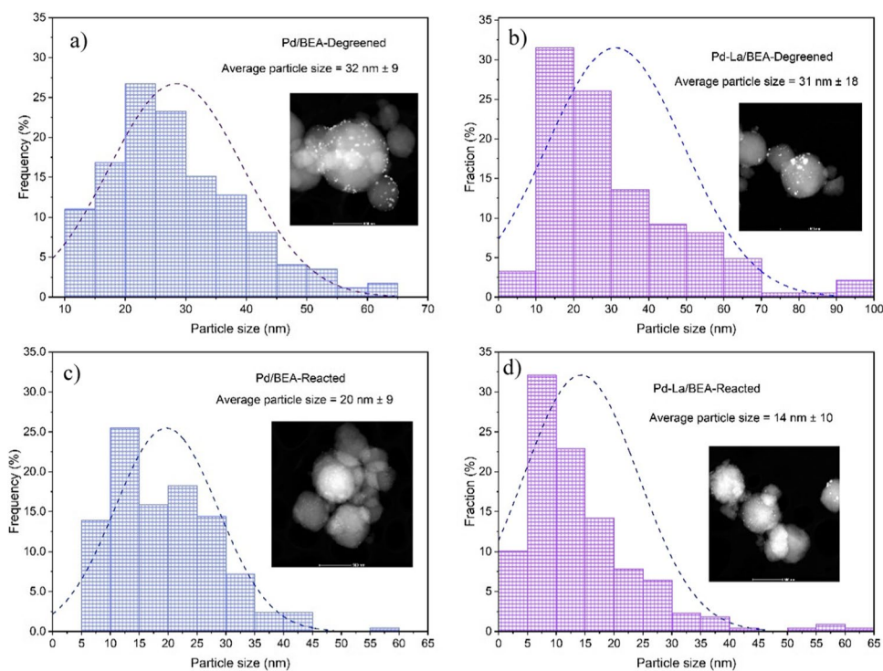
Fig. 3 STEM images and particle size fraction for degreened a Pd/BEA, b Pd-La/BEA and reacted c Pd/BEA, d Pd-La/BEA
