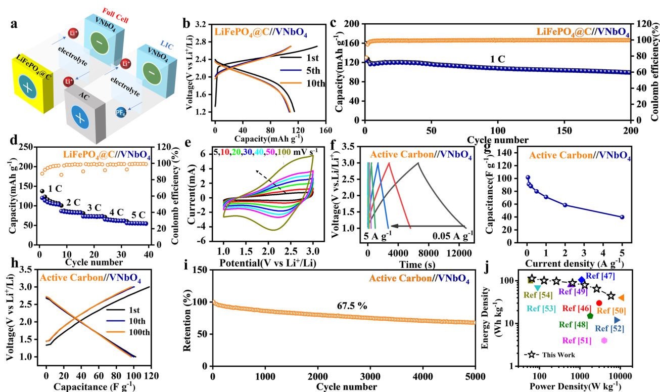
Fig. 6 a Models diagram of \text{LiFePO}_4@C/\text{VNbO}_4 full cell and \text{AC}/\text{VNbO}_4 LIC. b The selected charge/discharge profiles, c the cycle performance at 1C, d the rate performance of \text{LiFePO}_4@C/\text{VNbO}_4 . e CV curves at different sweep rates (5–100 \text{mV s}^{-1} ) and f the time-potential curves at different current densities of \text{AC}/\text{VNbO}_4 . g Rate performance, h the selected charge/discharge profiles at 0.05 \text{ A g}^{-1} , and i the cycle performance at 0.5 \text{ A g}^{-1} of \text{AC}/\text{VNbO}_4 . j The Ragone plot of \text{AC}/\text{VNbO}_4 compared with other reported niobium-based LICs
