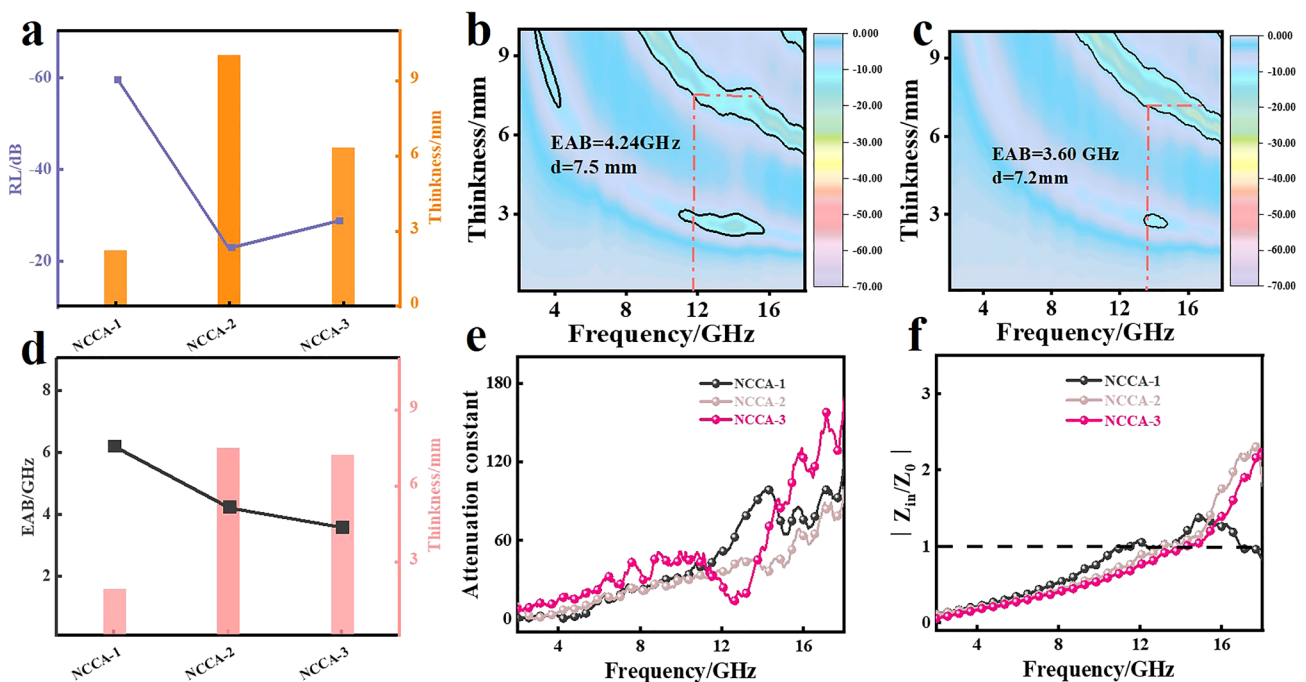
Fig. 5 a RL and corresponding matching thickness of NCCA-1, NCCA-2, NCCA-3. b , c 2D RL diagram of NCCA-2, NCCA-3. d EAB and corresponding matching thickness of NCCA-1, NCCA-2, NCCA-3. e Attenuation constant and f impedance matching of NCCA-1, NCCA-2, NCCA-3
