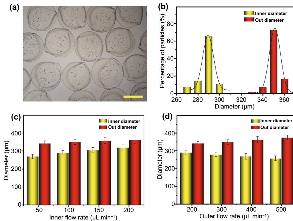
Fig. 3 Factors controlling the microcapsules size. a, b The morphology ( a ) and size distribution ( b ) of produced microcapsules. c, d The relationship of inner ( c ) and outer ( d ) phase flow rates on microcapsules size. The scale bar is 200 µm
