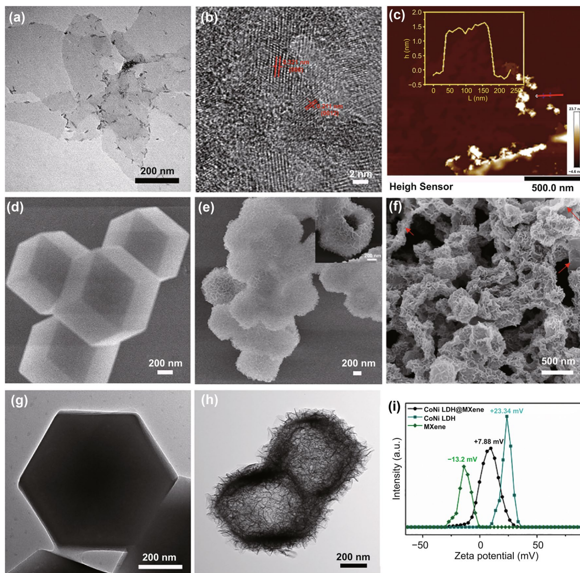
Fig. 2 a TEM, b HRTEM, c AFM images of \text{Ti}_3\text{C}_2\text{T}_x nanosheets. d SEM, g TEM images of ZIF-67 precursors. e SEM, h TEM images of NiCo LDH nanocage. f SEM image of hollow LDHT nanostructure. i Zeta potentials image of \text{Ti}_3\text{C}_2\text{T}_x suspension, NiCo LDH and LDHT
