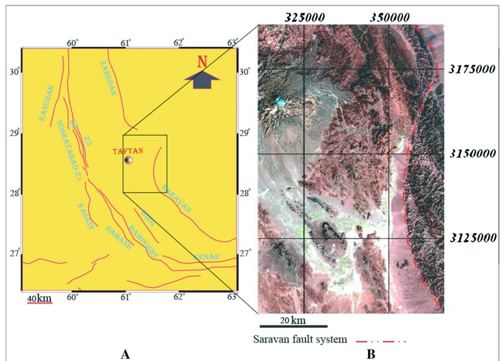
Fig. 2 a Graphical layout of main faults around the study area. b Landsat (TM) image from study area in the east of Taftan volcano and curvature of Saravan fault
