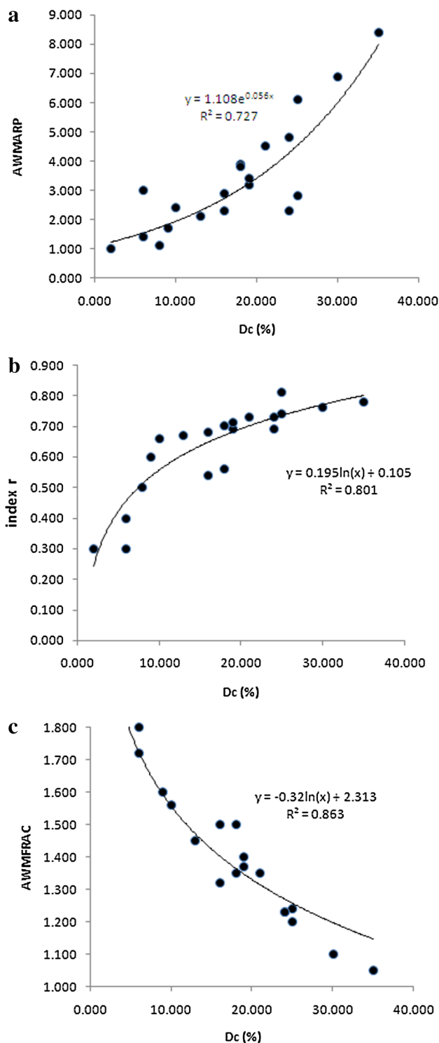
Fig. 4 Regression model for the soil cracks morphology
