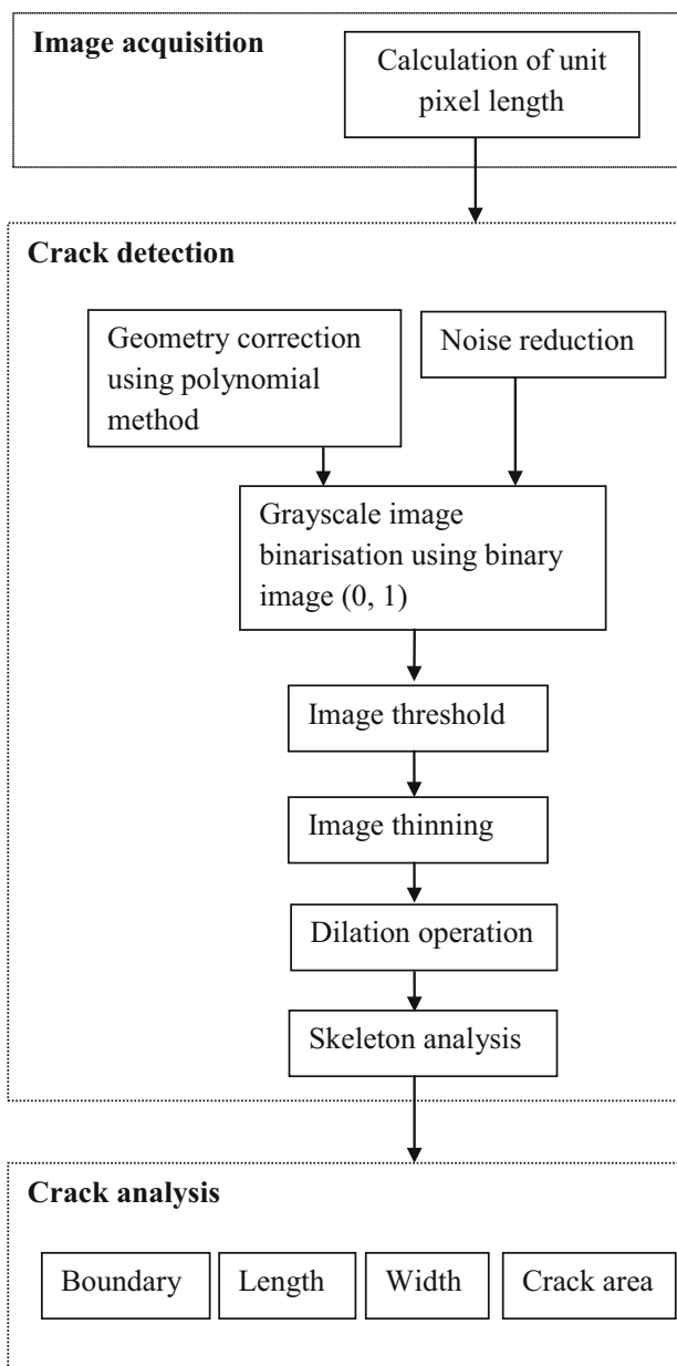
Fig. 2 Flowchart of the methodology (after modified Lee et al. 2013)
