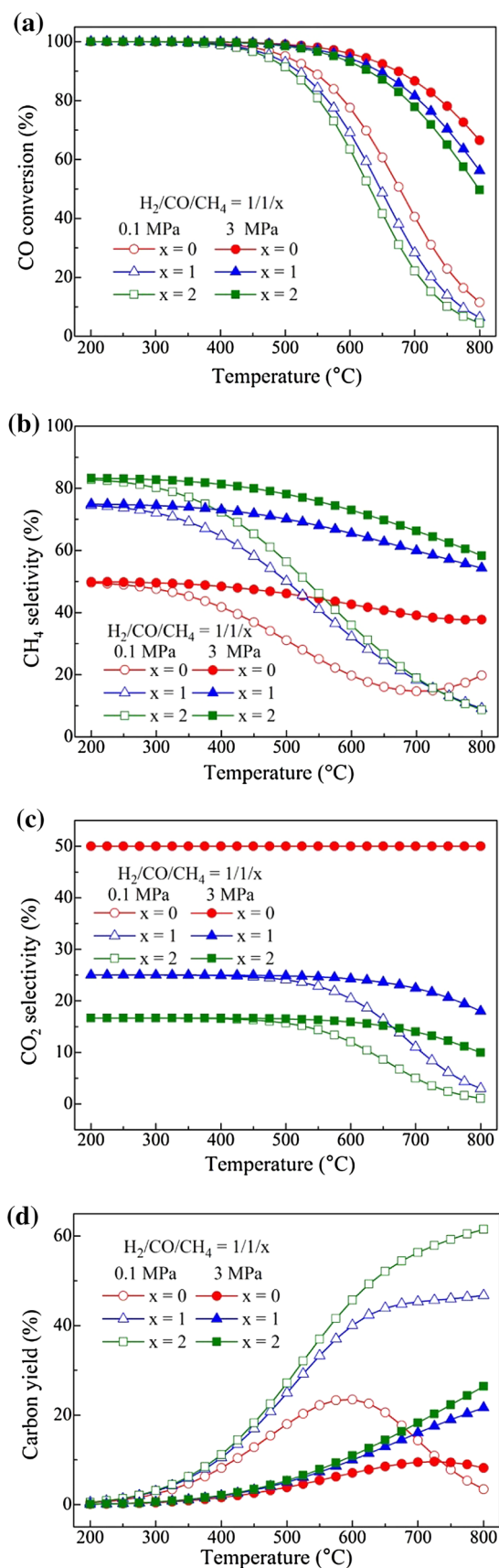
Fig. 6 Effect of CH 4 imputed into the feed gas on catalytic performance. a CO conversion, b CH 4 selectivity, c CO 2 selectivity, and d carbon yield
