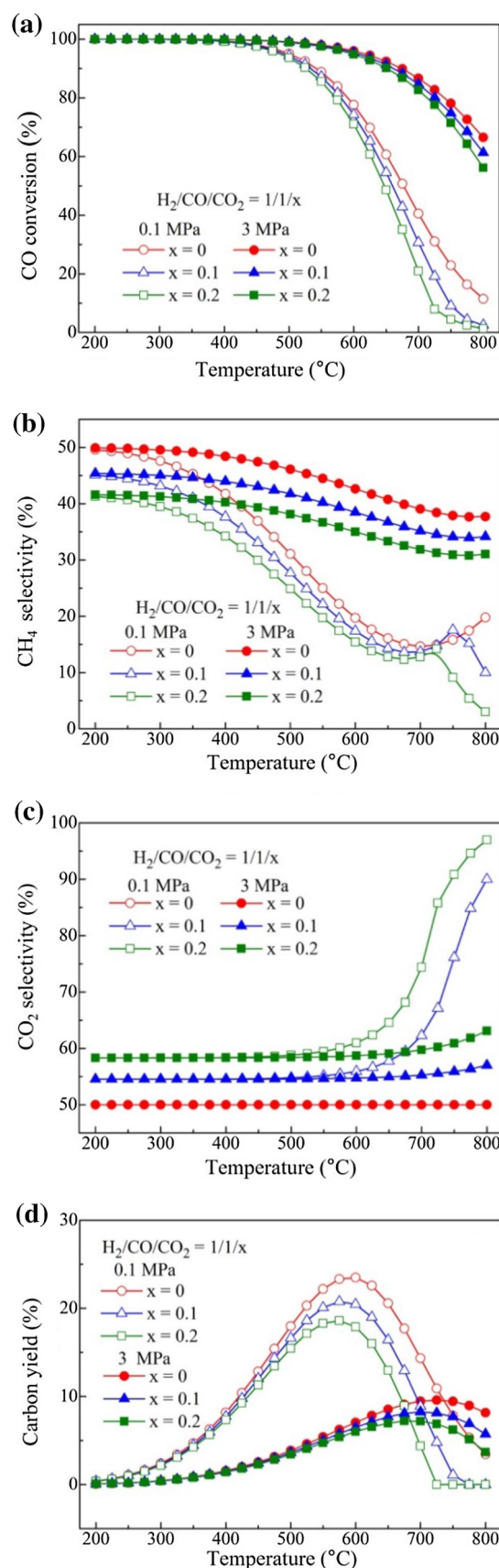
Fig. 7 Effect of \text{CO}_2 introduced into the feed gas on catalytic performance. a CO conversion, b \text{CH}_4 selectivity, c \text{CO}_2 selectivity, and d carbon yield
