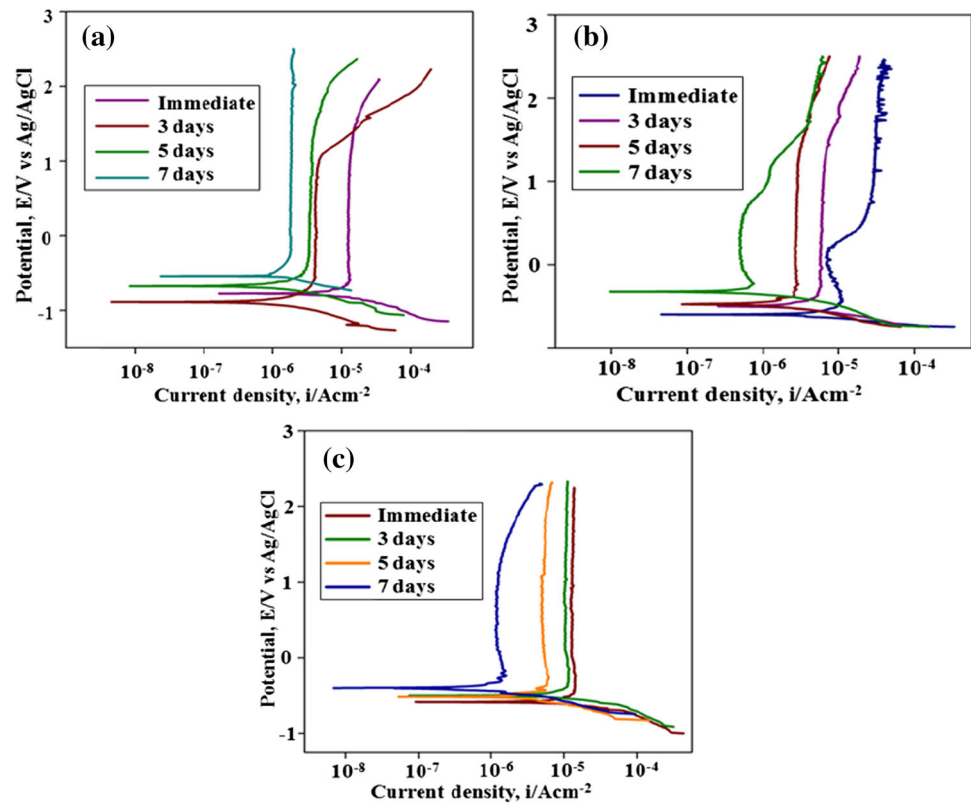
Fig. 13 Polarization curves of a TNT, b TNT with Sr and c TNT with Zr after immediate, 3, 5, and 7 days of immersion in Hank's solution
