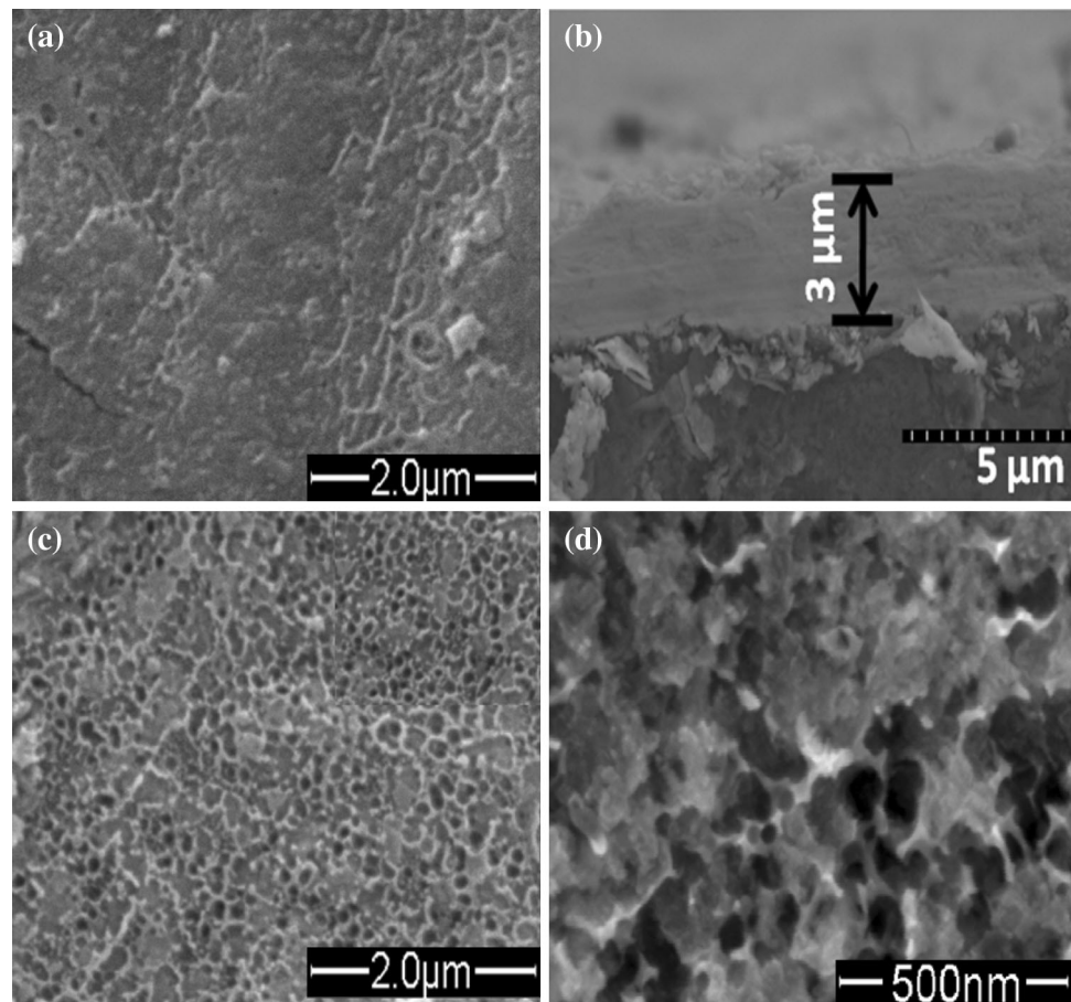
Fig. 5 SEM images of the anodized Ti at 40 V in 0.13 M H_2SO_4 with different HF concentrations: a 0.1 M HF, b cross-sectional view c 0.15 M HF and d 0.2 M HF
