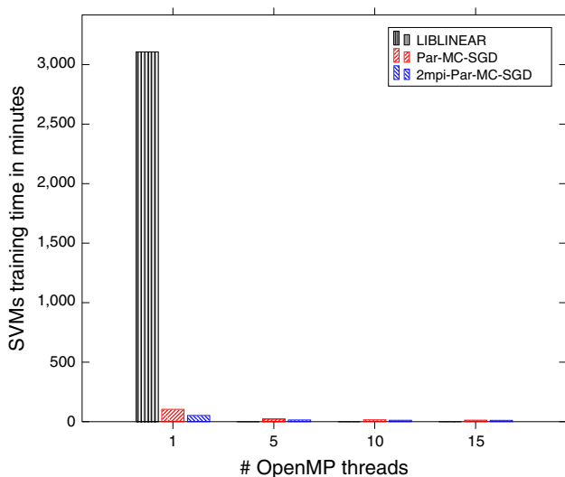
Fig. 5 SVMs training time with respect to the number of threads on ILSVRC 2010
