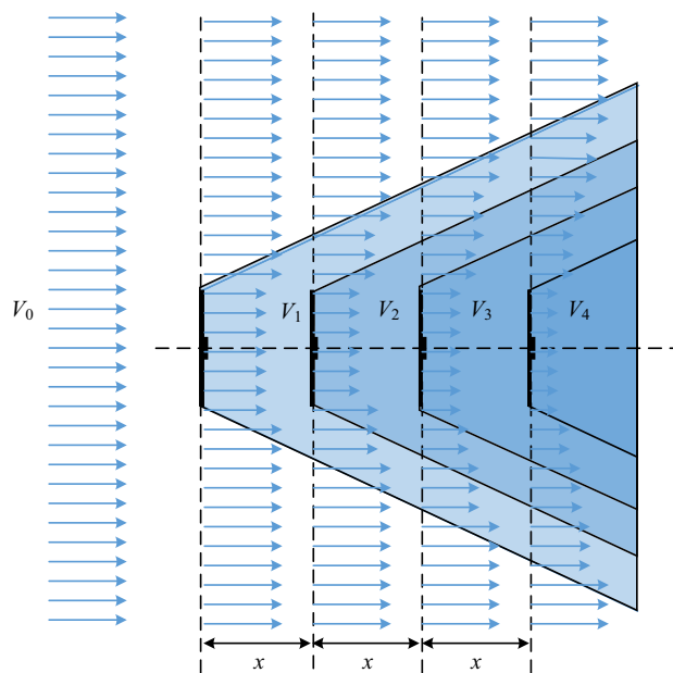
(a) Several WTs in a line
