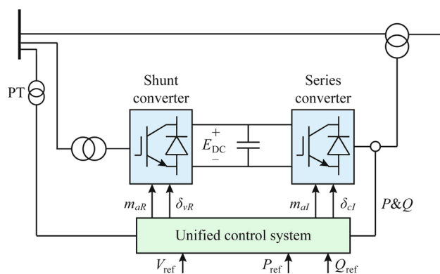
Fig. 13 UPFC schematic representation
