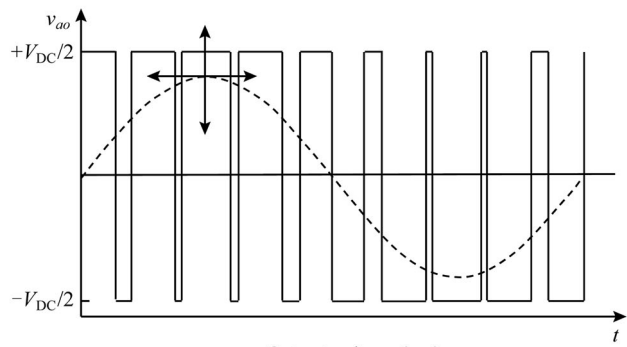
(b) Synthesized AC voltage
