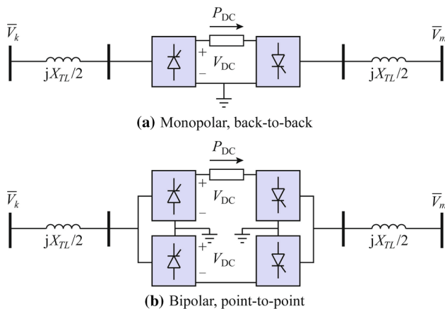
Fig. 14 HVDC systems
