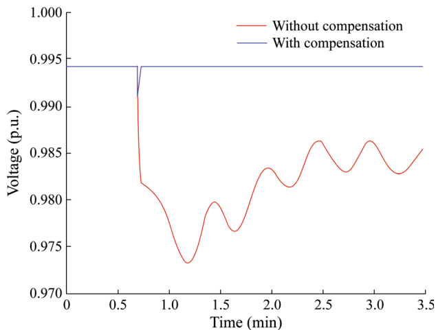
Fig. 22 Dynamic stability improvement: comparison of voltage evolution in a transmission line with and without shunt compensation at midpoint during a transient due to a load increase
