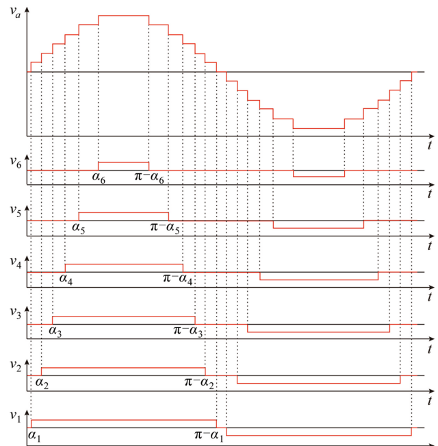
(b) Synthesized AC voltage
