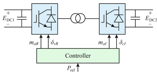
Fig. 17 DC/DC converter based on VSCs
