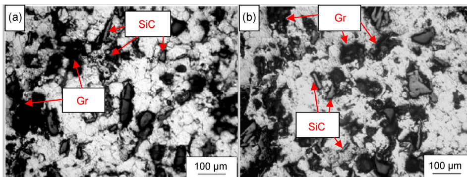
Fig. 4 Optical micrographs of fabricated composites (a) Al2024/5%SiC/5%Gr and (b) Al2024/5%SiC/10%Gr composites. Reproduced with permission from Ref. [52]. Copyright Elsevier, 2012.
