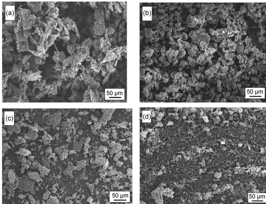
Fig. 15 SEM micrographs of the collected debris from (a) nano-Al2024, (b) nano-Al/5%SiC, (c) nano-Al/5%SiC/5%Gr, and (d) nano-Al/5%SiC/10%Gr. Reproduced with permission from Ref. [50]. Copyright Elsevier, 2013.
