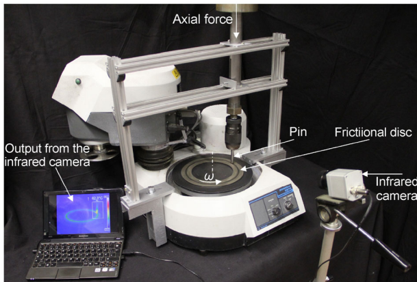
Fig. 7 Test rig and temperature measurement of a pin-on-disc test.
