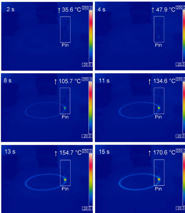
Fig. 8 Values of temperature which are calculated using infrared camera during the sliding operation.
