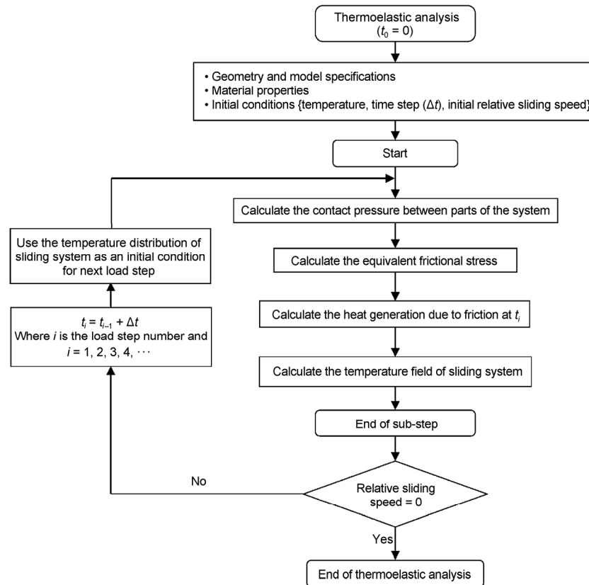
Fig. 2 Flowchart of finite element simulation of fully thermal-mechanical approach.
