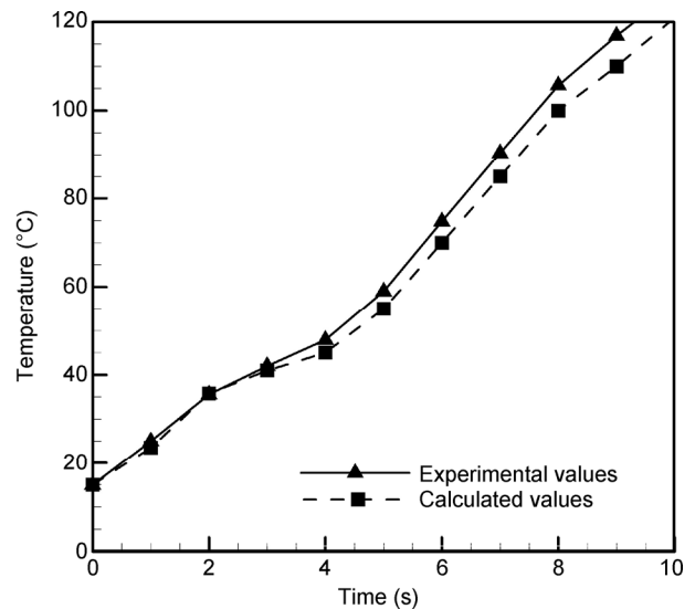
Fig. 9 History of the temperature during the sliding operation.
