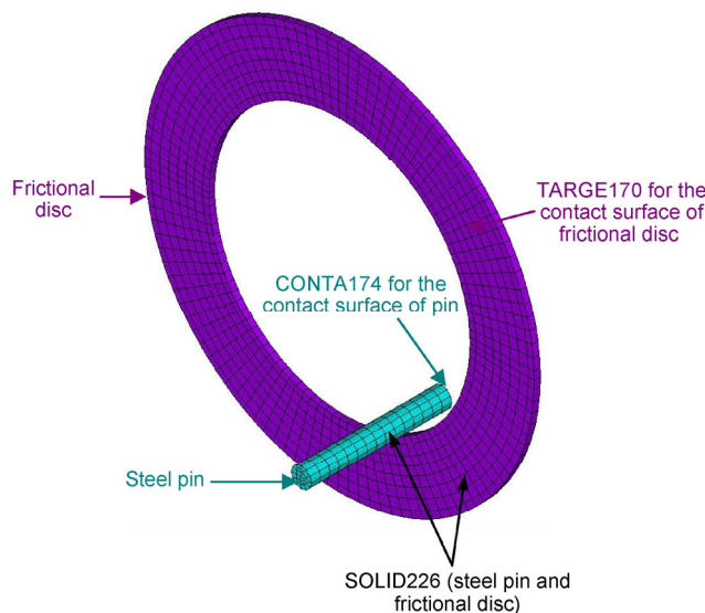
Fig. 4 Elements which used in the sliding simulation of a pin-on-disc test.
