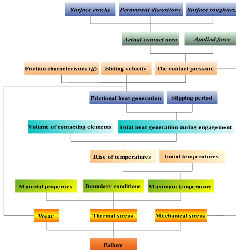
Fig. 1 Diagram of the effective variables on the thermo-mechanical behavior of dry sliding systems.
