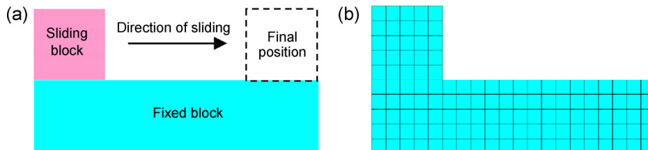
Fig. 3 FE model of block sliding over another fixed block [16]: (a) sliding model, (b) FE model (No. of total elements = 125).
