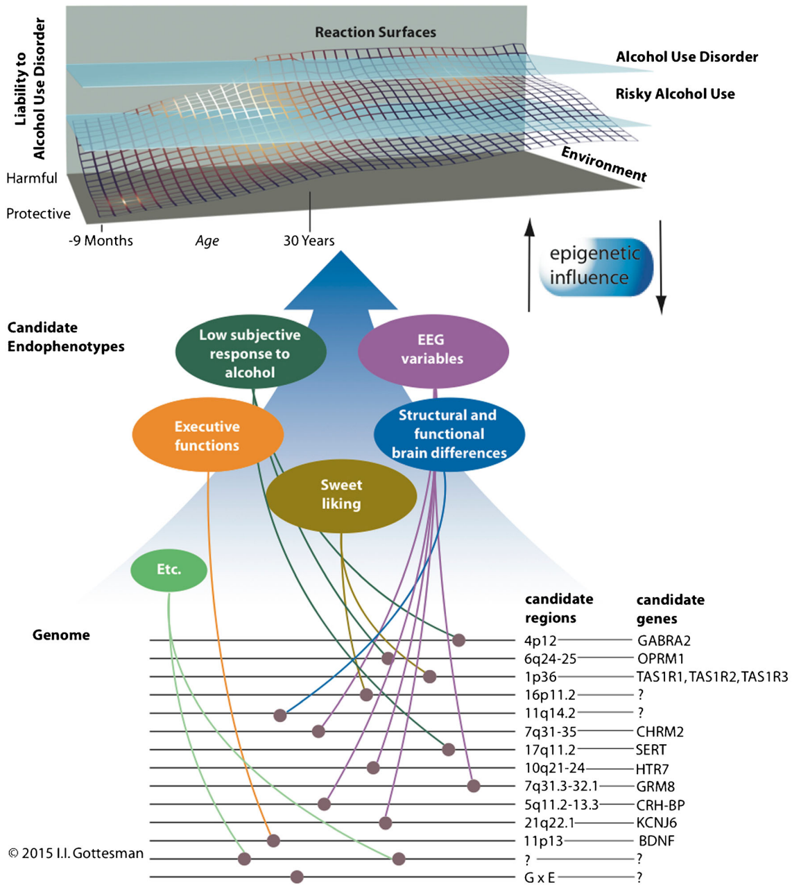
Fig. 1 Depiction of the interplay among genetic and environmental factors that contribute to liability for alcohol use disorder (AUD), and the contribution of candidate endophenotypes and their associated genes and gene regions. Genes and gene regions that are associated with AUD candidate endophenotypes are highlighted here (references are documented in Table 2). These should be considered illustrative and
