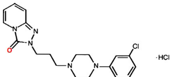
Fig. 1 Structural formula of trazodone
