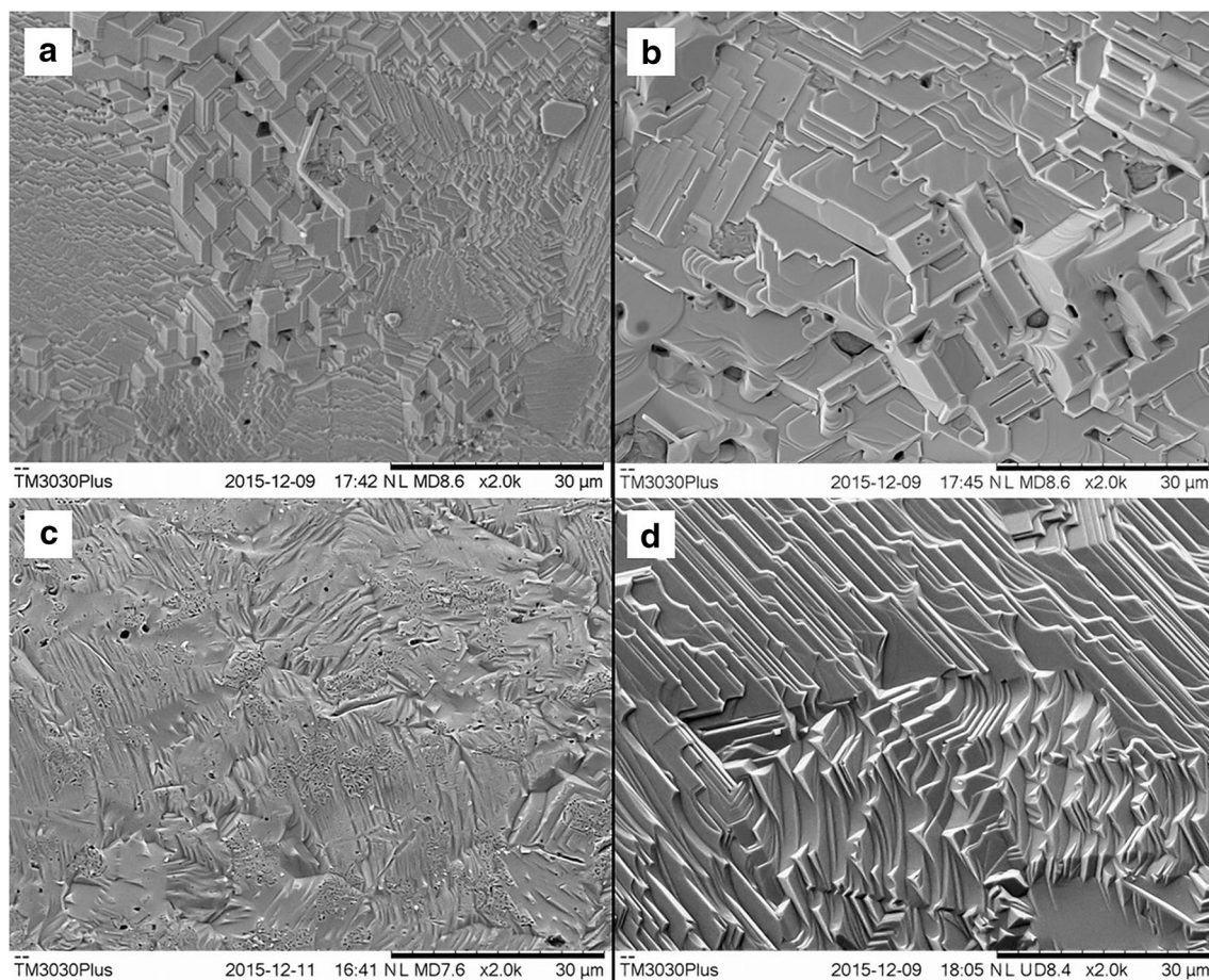
Fig. 5 SEM scans of the surface of Ag interconnect wire (1 cm from the cell) after test under constant current for 850 h at 650 °C: a, b cathode lead; c anode lead; d the surface of Ag cathode wire after 450 h at 700 °C
