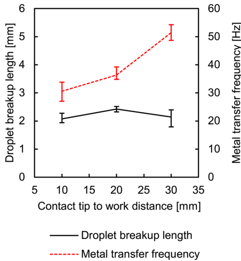
Fig. 9 Average droplet breakup length and metal transfer frequency as wire extensions increase in Group C
