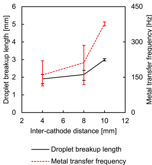
Fig. 7 Average droplet breakup length and metal transfer frequency as inter-cathode distances increase in Group B
