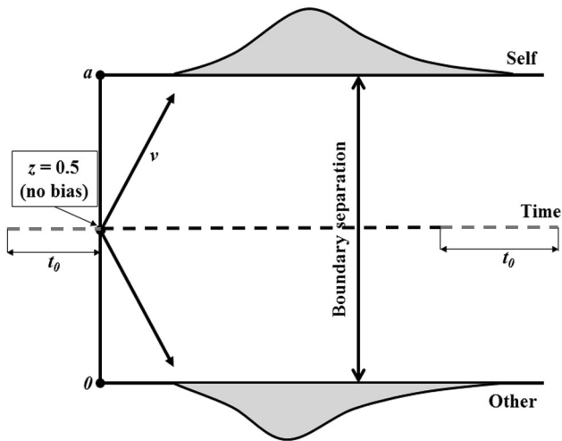
Fig. 1 Schematic representation of the drift diffusion model. An information gathering process begins at starting point z and continues with a mean slope v until it reaches an upper ( a ) or lower ( 0 ) threshold. Non-decision processes ( t_0 ) reflect how much time elapses before/after the decision process. The process durations and outcomes vary from trial to trial because of random noise. Outside the threshold boundaries the response distributions are shown
