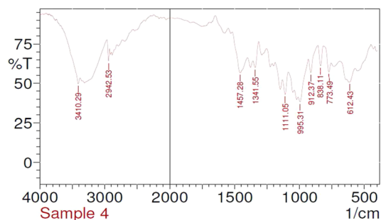
Fig. 7 FT-IR spectrum of ascorbic acid
