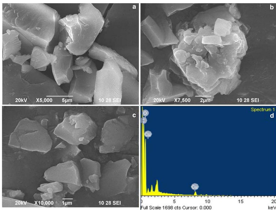
Fig. 3 Electron microscopic observation and elemental analysis of Chi–CuO nanocomposites, (a–c) SEM image of Chi–CuO nanocomposites and (d) EDX spectrum of Chi–CuO
