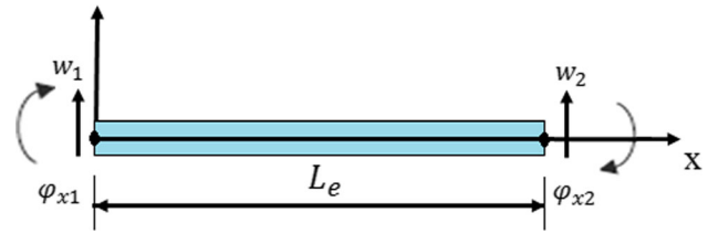
Fig. 1 Two degrees of freedom element beam
