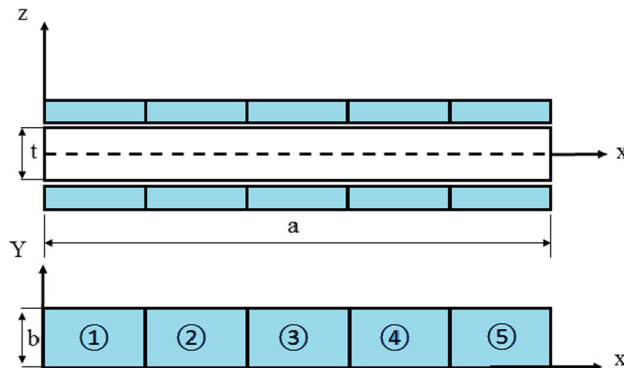
Fig. 3 A beam with surface-bonded piezoelectric actuators
