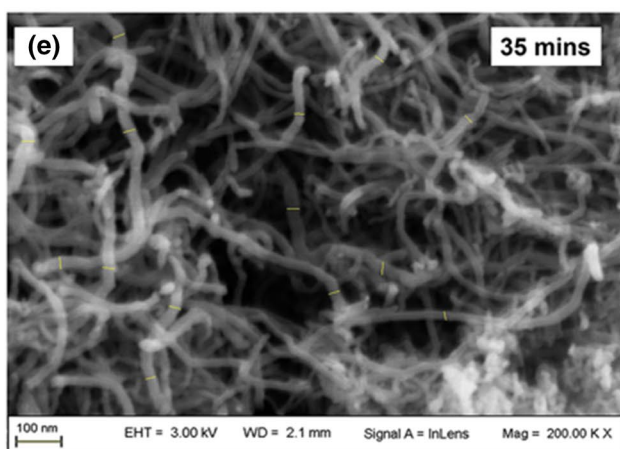
Fig. 6 FESEM image of MWCNTs grown at different processing time (a, c, e) and distribution of MWCNTs diameter as a function of processing time (b, d, f)
