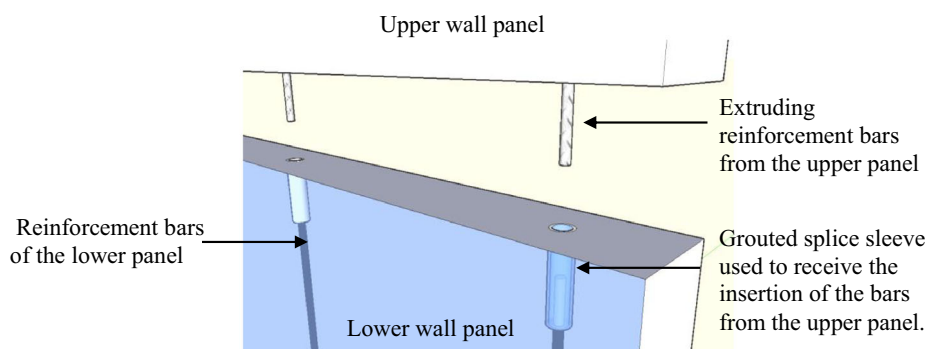
Fig. 3 Grouted splice sleeve as the connection of precast concrete wall panels (Loh 2008).
