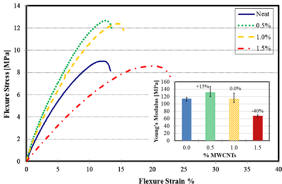
Fig. 6 Stress–strain curves of flexure test of PC with varying MWCNTs content. Inset shows the change in modulus of elasticity of PC with varying MWCNTs content.
