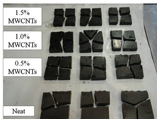
Fig. 8 Cracking pattern due to impact of PC with varying MWCNTs content.
