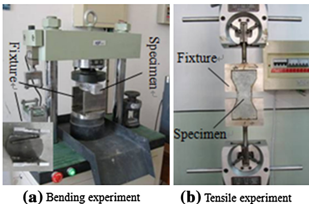
Fig. 3 Loading devices for bending and tensile tests.
