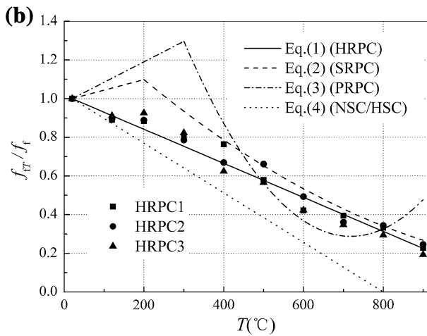
Fig. 6 Flexural strength of hybrid fiber-reinforced RPC after exposure to elevated temperatures. a Absolute value. b Relative value.
