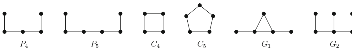
Fig. 1 Graphs P_4, P_5, C_4, C_5, G_1 and G_2
