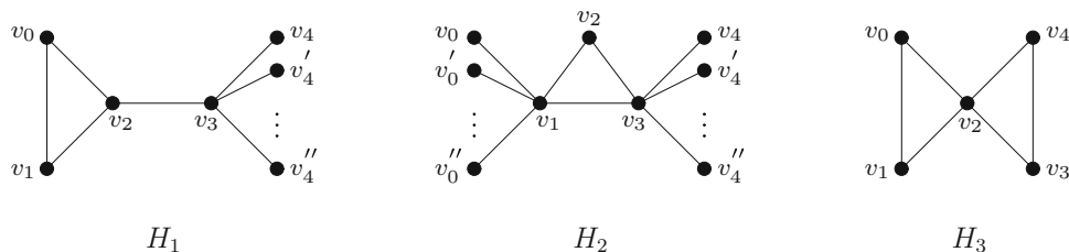
Fig. 2 Graphs H_1, H_2 and H_3
