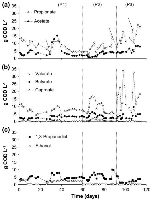
Fig. 2 General distribution of carboxylates (a) and (b), ethanol and 1,3-propanediol (c) concentrations throughout the three operational phases (P1), (P2), and (P3)
