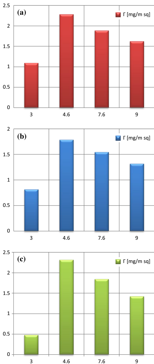
Fig. 5 The albumin amount adsorbed on the Cr 2 O 3 particles as a function of solution pH: a BSA, b OVA, c HSA. C albumin (initial) = 250 ppm
