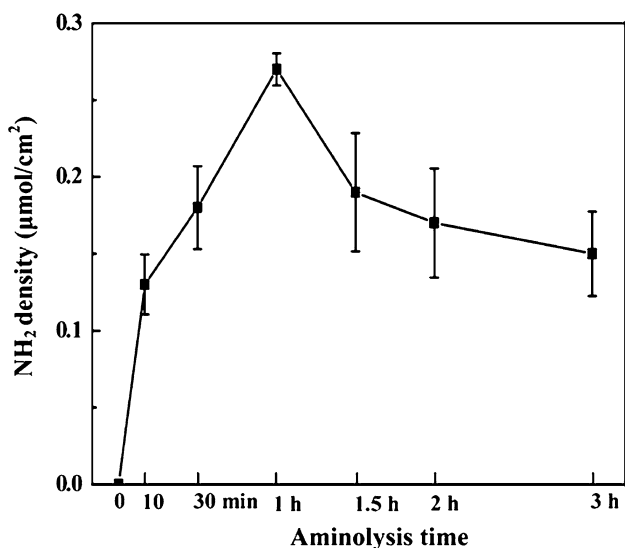
Fig. 1 The density of amine groups of the aminolyzed PCL film surface as a function of aminolysis time as determined by the ninhydrin assay. The analysis reaction of PCL films proceeded at 40 °C in 10 wt% 1,6-hexanediamine/2-propanol solution. Error bars represent the standard deviation over three separate PCL films. The optimized aminolysis time was observed at 1 h with NH 2 density at about 0.265 \mu\text{mol}/\text{cm}^2
