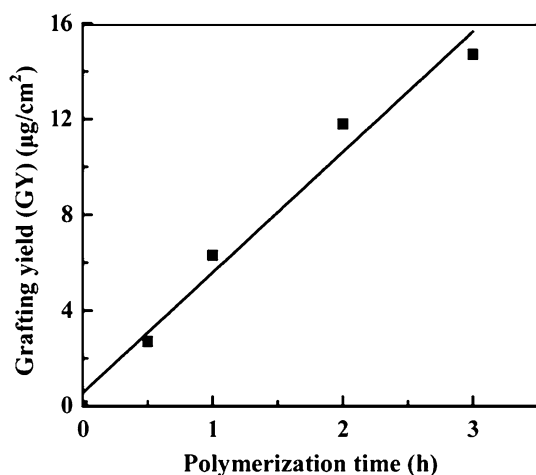
Fig. 5 A linear relationship between the grafting yield (GY) of the P(GMA) brushes with the surface-initiated ATRP time was observed. The polymer chain growth from the PCL-Br surface could be controlled by varying reaction time
