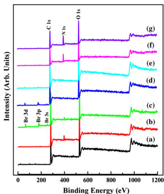
Fig. 3 Wide scan XPS spectra of the a pristine PCL, b PCL-NH 2 from 1 h of aminolysis, c PCL-Br, d PCL- g -P(GMA)1 from 1 h of ATRP, e PCL- g -P(GMA)2 from 3 h of ATRP, f PCL- g -P(GMA)1- c -gelatin, and g PCL- g -P(GMA)2- c -gelatin surfaces
