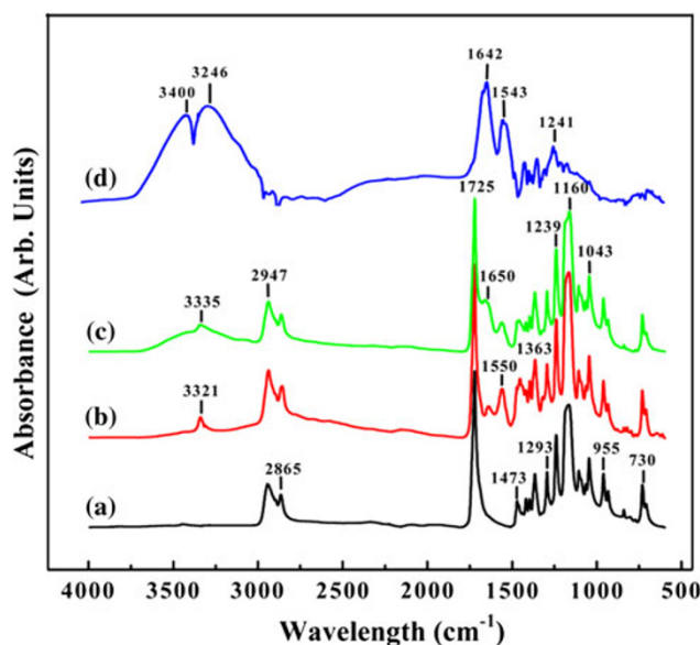
Fig. 2 ATR-FTIR spectra of the a pristine PCL, b PCL-NH 2 from 1 h of aminolysis, c PCL-gelatin, d pure gelatin. The successful immobilization of gelatin was deduced from the presence of a broad band of free O-H and N-H groups (at 3,295 \text{ cm}^{-1} ), amide I band (at 1,650 \text{ cm}^{-1} ) and amide II band (at 1,550 \text{ cm}^{-1} ) as compared to the FTIR spectrum of pure gelatin
