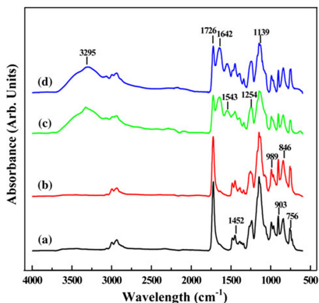
Fig. 4 ATR-FTIR spectra of the a PCL- g -P(GMA)1 from 1 h of ATRP, b PCL- g -P(GMA)2 from 3 h of ATRP, c PCL- g -P(GMA)1- c -gelatin, and d PCL- g -P(GMA)2- c -gelatin. The successful immobilization of gelatin on the P(GMA) brushes can be deduced from the presence of a broad band of free O-H and N-H groups (at 3,295 \text{cm}^{-1} ), amide I band (at 1,642 \text{cm}^{-1} ) and amide II band (at 1,543 \text{cm}^{-1} ) as compared to the pure gelatin FTIR spectrum
