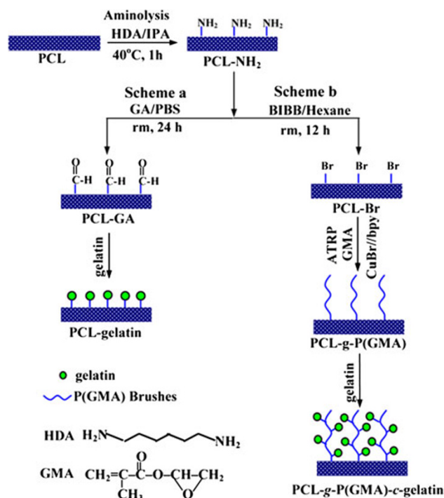
Scheme 1 Schematic diagram illustrating the aminolysis process used to introduce free amino groups to PCL (i.e. PCL-NH 2 surface) and the two subsequent surface-modification schemes used to create gelatinized substrates. In scheme a, gelatin is covalently immobilized onto the aminolyzed PCL surface with glutaraldehyde as a cross-linking agent, resulting in the PCL-gelatin surface. In Scheme b, immobilization of an alkyl bromine-containing initiator via condensation reaction leads to the formation of the PCL-Br surface. Surface-initiated ATRP of GMA from the PCL-Br surface results in the formation of the PCL-g-P(GMA) surface, and subsequently covalent conjugation of gelatin will result in the PCL-g-P(GMA)-c-gelatin surface
