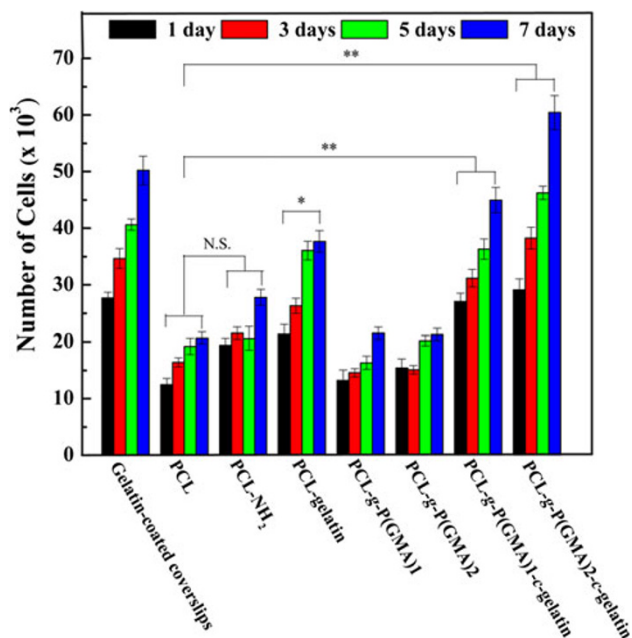
Fig. 6 Cell proliferation profile of the gelatin-coated coverslips, pristine PCL and functionalized PCL surfaces after 1, 3, 5 and 7 days of incubation at 37 °C in a 5 % CO 2 atmosphere as determined by the AlamarBlue™ (AB) assay. Data is presented as means ± SD. * p < 0.05, ** p < 0.01 compared to the pristine PCL substrates. The proliferation rate of HUVECs seeded on the PCL-g-P(GMA)- c -gelatin surfaces was significantly improved as compared to the pristine PCL and PCL-g-P(GMA) film surfaces
