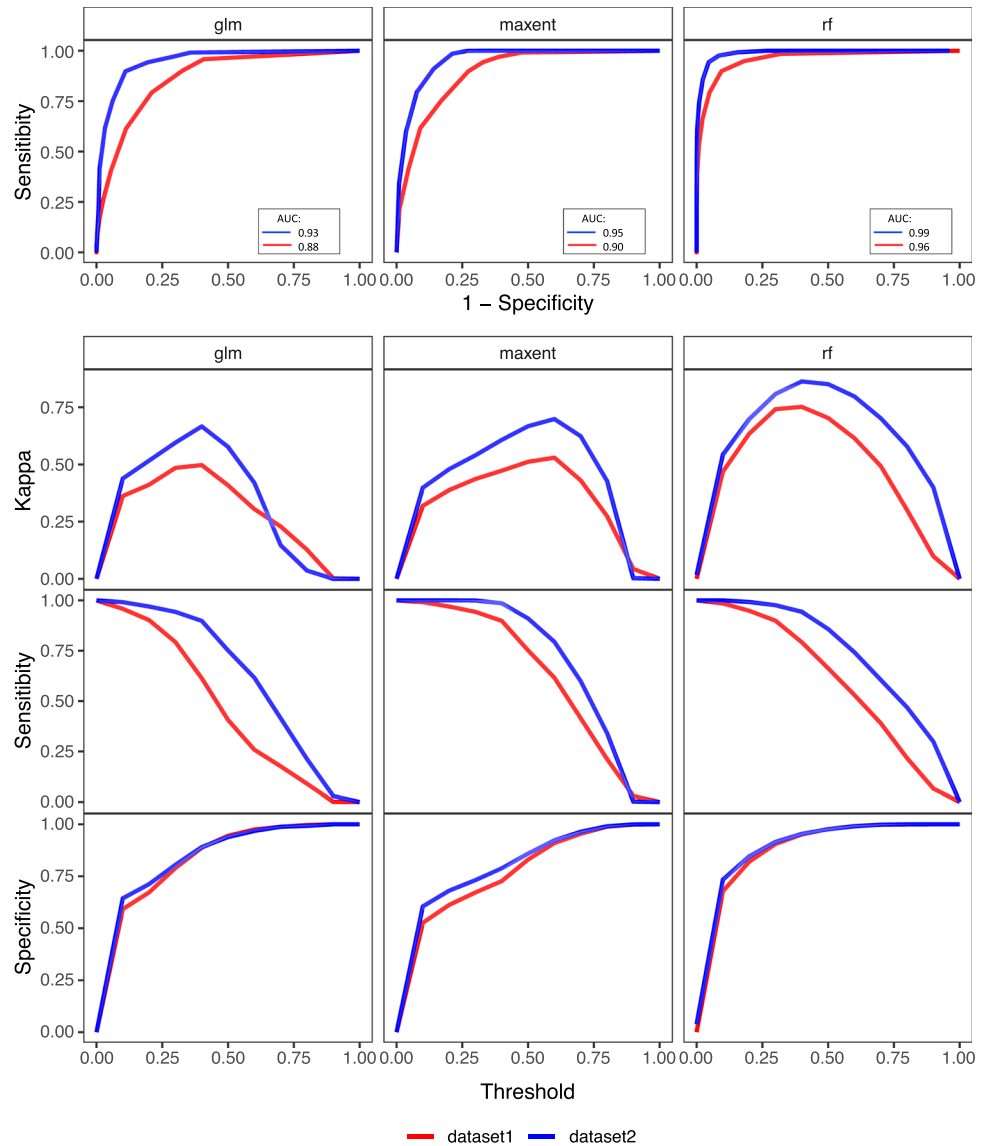
Fig. 2 Mean values and standard deviations of threshold independent (AUC) and dependent (kappa, sensitivity, and specificity) measures of discrimination for the 10 models for dataset 1 (red) and dataset 2 (blue) for each method. Generalized linear models (GLM), random forest (RF), and maximum entropy (Maxent)
