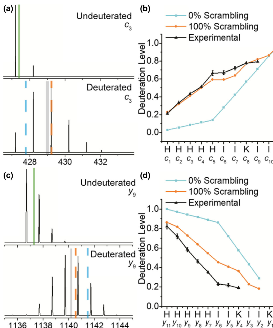
Figure 2. Observed isotopic distributions of c_3 (a) and y_9 (c) fragment ions from nCID of the natural and deuterated peptide P1 (HHHHHHHIIKLIK). The weighted average m/z value for each species is illustrated by a solid green (natural) or gray (deuterated) line. Theoretical deuterium levels for 100 and 0% scrambling are denoted with dashed orange (100%) and blue (0%) lines, respectively. Deuterium levels for all measured P1 nCID-derived c - (b) and y -type (d) fragment ions. Blue and orange lines represent expected deuterium levels for 0 and 100% scrambling, respectively
