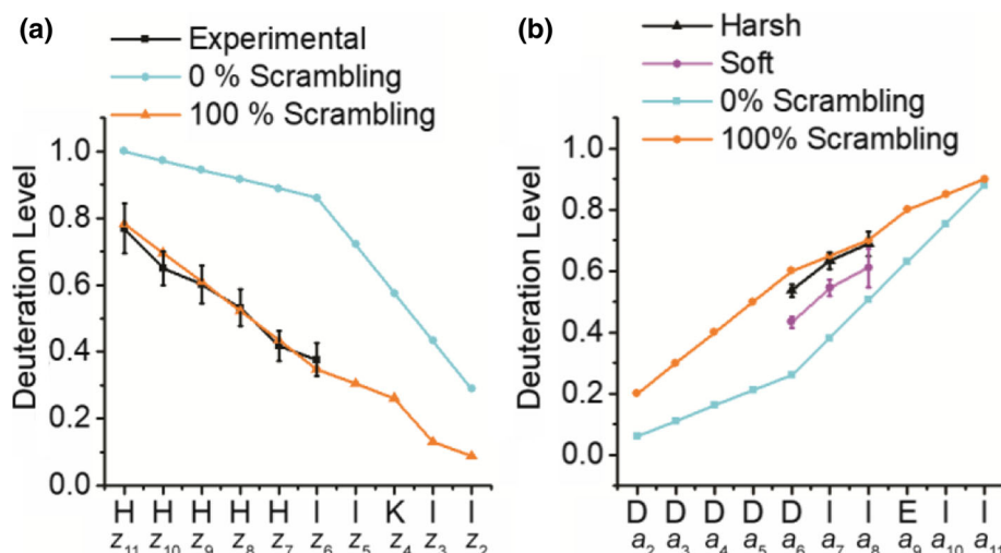
Figure 5. Deuteration levels of nFRIPS-generated z -type fragment ions (a) and EDD-generated a -type ions (b) from the peptide P3, as well as predicted 0 and 100% scrambling curves. EDD was performed after both “soft” and “harsh” ion source conditions
