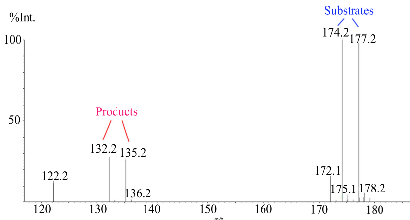
Figure 2. Spectrum of simultaneous enzymatic catalysis. Appearing simultaneously in one spectrum, the peaks of isotope substrates and isotope products show that isotope substrates have similar hydrolysis rate. (In the spectrum, m/z = 177.2 and 174.2 are peaks of isotope substrates; m/z = 135.2 and 132.2 are peaks of isotope products; m/z = 122.2 is peak of [\text{Tris}+\text{H}]^+ because the enzyme powder was lyophilized in Tris-HCl buffer before reconstitution)
