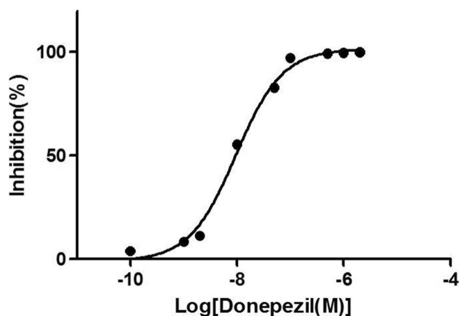
Figure 3. Plot of the inhibition efficiency of donepezil hydrochloride toward AChE. The concentration of light-isotope/heavy-isotope substrates were 0.05 mg/mL and AChE concentration was fixed at 0.1 U/mL
