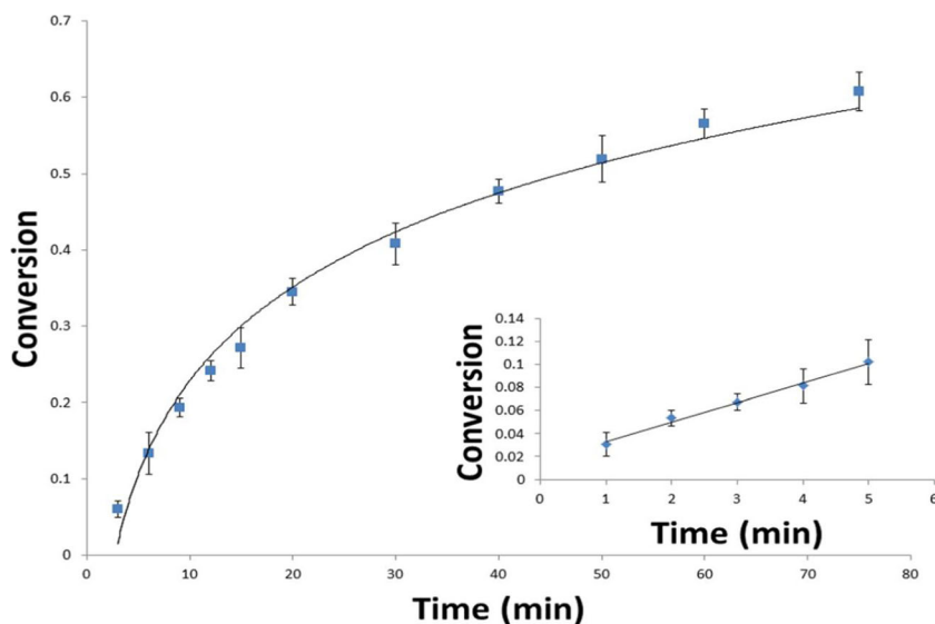
Figure 1. Progress curves of enzyme-catalyzed reaction. The initial substrate concentration was 0.2 mg/mL; the reaction was quenched at 3, 6, 9, 12, 15, 20, 30, 40, 50, 60, and 75 min by the addition of acetonitrile (200 \mu L); to fully demonstrate the accuracy of the linear correlation between conversion and time before 5 min, experiments of time data acquisitions are added below 5 min
