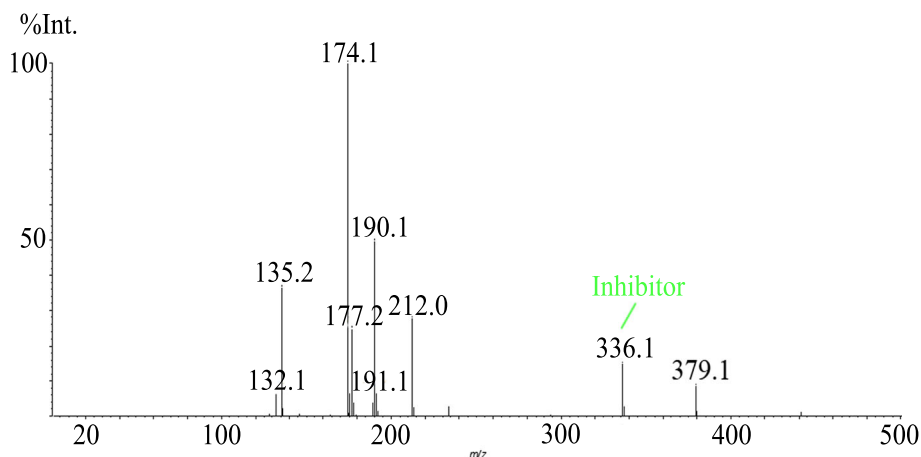
Figure 4. The mass spectrum for screening inhibitors from crude Phellodendron chinense Schneid. extracts. The active ingredient, Majorine (exact mass = 336.1230), can be shown in the spectrum. (In the spectrum, m/z = 177.2 and 174.2 are peaks of isotope substrates; m/z = 135.2 and 132.2 are peaks of isotope products; m/z = 190.1 , 212.0 , and 379.1 are peaks of CHCA matrix)
