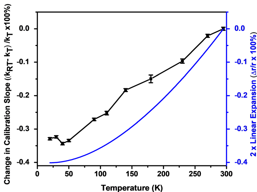
Figure 6. The relative difference of calibration slopes relative to room temperature (black) is plotted alongside with the thermal contraction of the trap radius [50] multiplied by 2 (blue)
