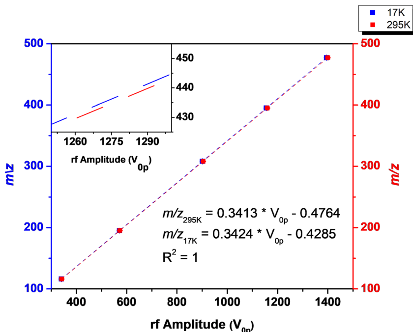
Figure 5. The mass calibration plots for room-temperature (red) and cryogenic-temperature (blue) mass instability scans. Linear regression fit lines are shown. The inset shows a blown-up view of the 1250–1300 V region to illustrate the difference in slope
