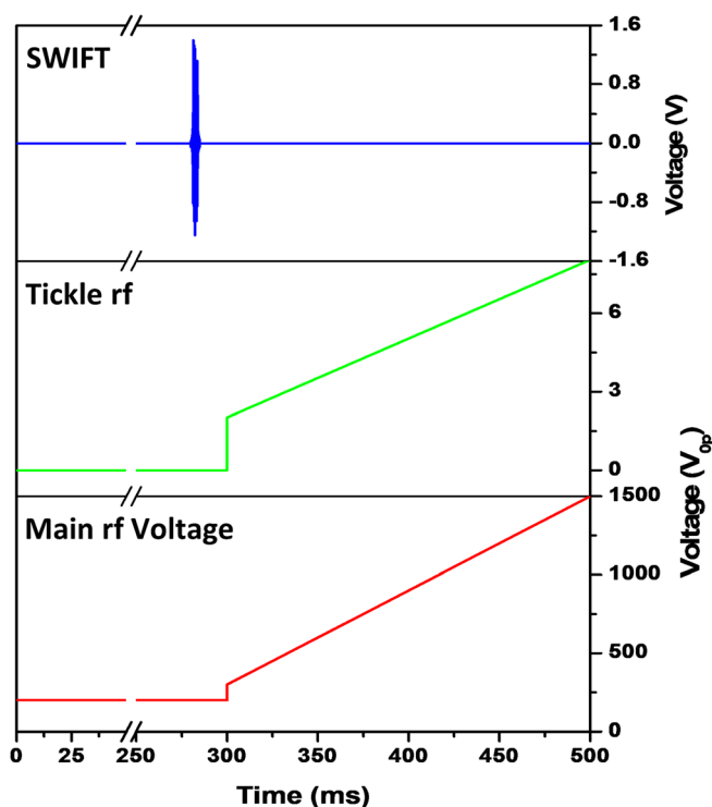
Figure 2. Experimental scheme for the mass instability scans. A SWIFT waveform is applied 20 ms before the scan, for 5 ms. during the mass scan, both the resonant auxiliary frequency and the main rf amplitude are ramped up
