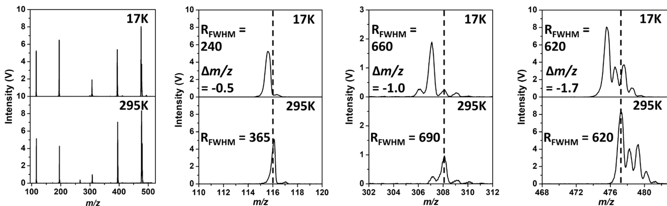
Figure 4. Comparison between the room temperature (295 K) (bottom) and cryogenic (top) mass spectra. The mass shift is more pronounced at higher masses as shown in the zoomed portions of the mass spectra (right)
