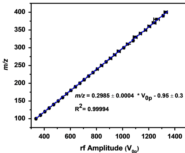
Figure 3. SIMION-simulated mass calibration curve, the mean rf amplitude, and standard deviation needed to eject a particular m/z , from the cryoLIT, from triplicate measurements. A_2 is calculated from the linear fit slope
