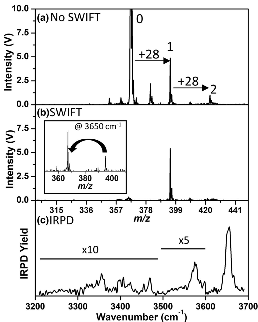
Figure 8. (a) Mass spectrum of GYK and its singly (1) and doubly (2) N_2 -tagged ions. (b) SWIFT-isolated mass spectrum of the singly N_2 -tagged GYK ion. The inset shows the mass spectrum after the loss of the nitrogen tag upon absorption of an IR photon at 3650\text{ cm}^{-1} . (c) Infrared predissociation spectrum of the singly tagged GYK ion
