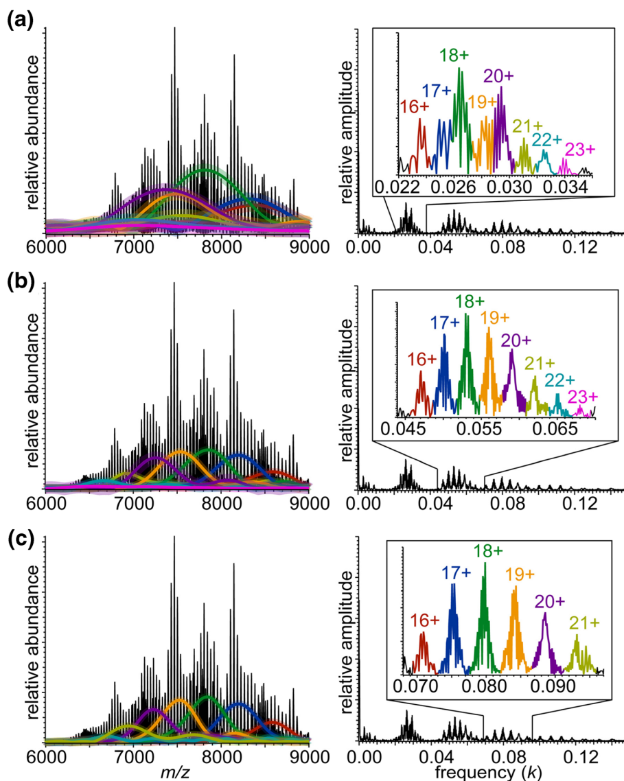
Figure 4. Mass spectrum of DMPC-MSP1D1 Nanodiscs acquired on an Orbitrap mass spectrometer (left) and corresponding Fourier spectrum (right) for (a) fundamentals, (b) second harmonics, and (c) third harmonics. IFT of the charge-state specific peaks in Fourier spectra (insets) are shown as overlaid envelope functions of the same color in mass spectra. Faint color surrounding envelope functions represents uncertainty of envelope functions calculated from average noise amplitude in the Fourier domain
