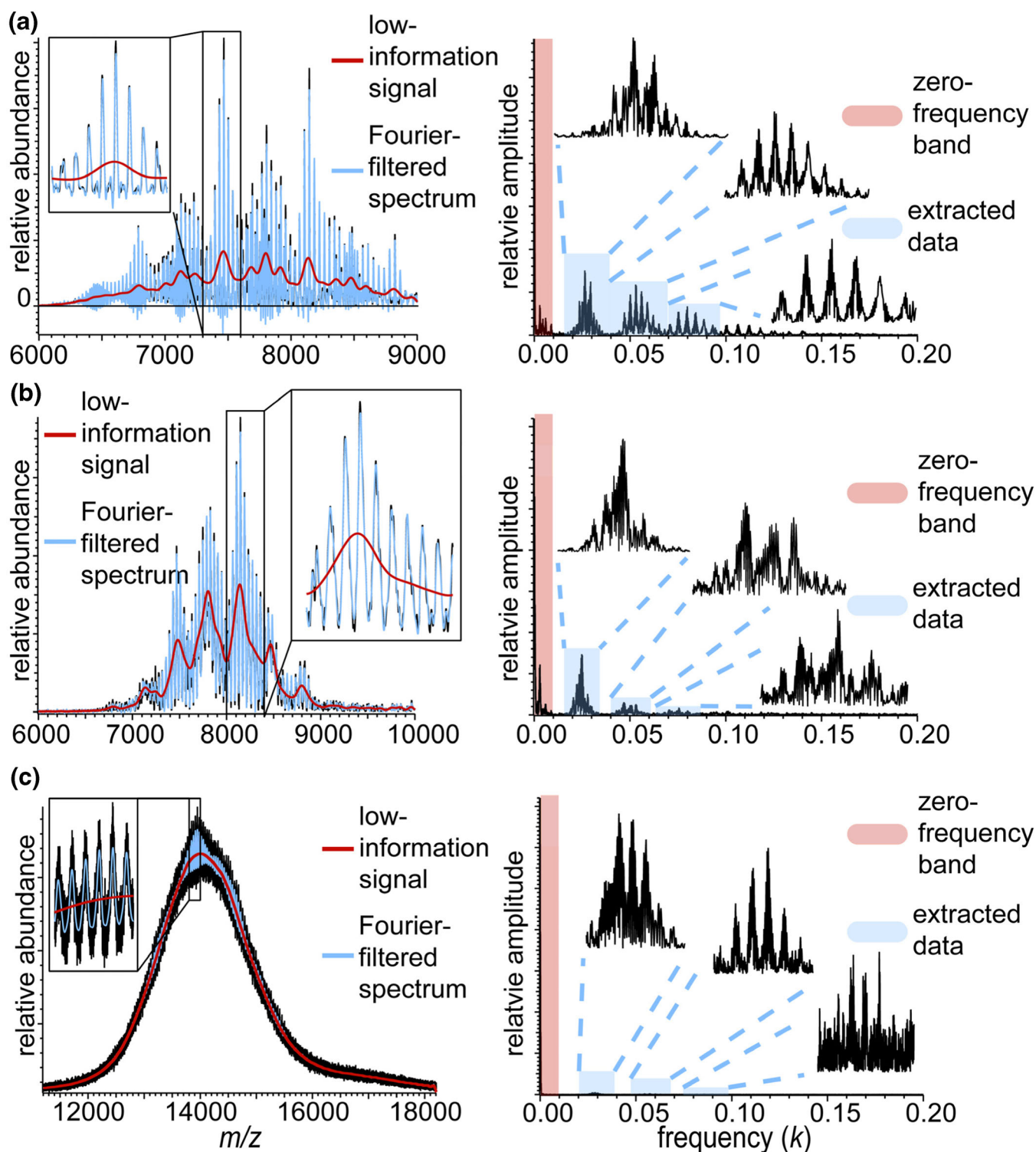
Figure 3. Mass spectra (left) and corresponding Fourier spectra (right) for native-like DMPC-MSP1D1 Nanodiscs measured on (a) Orbitrap and (b) FT-ICR mass spectrometers, and (c) a DPPC-MSP1E3D1 Nanodisc mass spectrum measured on a QTOF mass spectrometer. Fourier-filtered mass spectra (blue overlays) are calculated using the first three harmonics, as well as the Fourier baseline (red) the corresponding to the zero-frequency band. Detailed peak structure illustrated in insets
