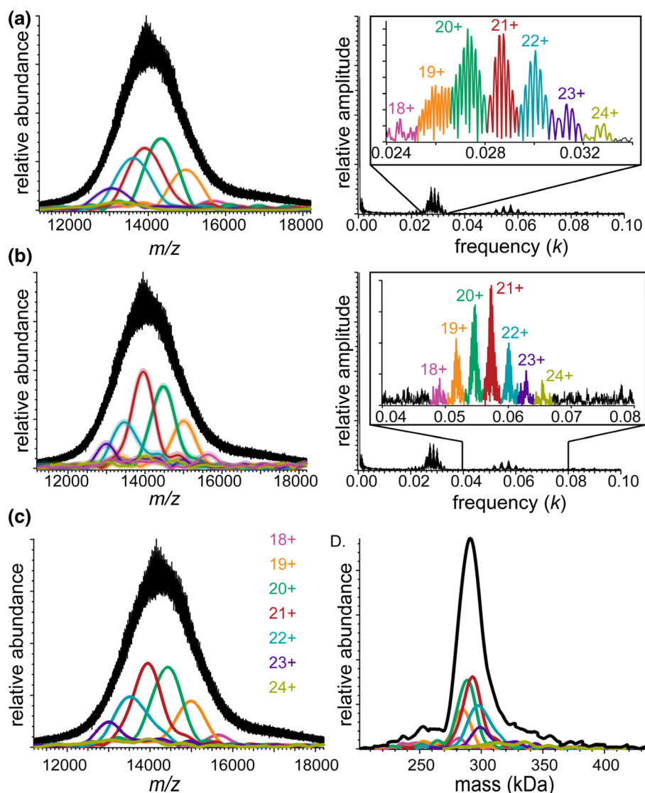
Figure 5. Mass spectrum of DPPC-MSP1E3D1 Nanodiscs acquired on a QTOF mass spectrometer (left) and corresponding Fourier spectrum (right) for (a) fundamentals and (b) second harmonics. IFT of the charge-state specific peaks in Fourier spectra (insets) are shown as overlaid envelope functions of the same color in mass spectra. Faint color surrounding envelope functions represents uncertainty of envelope functions calculated from average noise amplitude in the Fourier domain. (c) Harmonic-averaged reconstruction of envelope functions. (d) Zero-charge spectrum (black), calculated from harmonic-averaged spectra for all charge states
