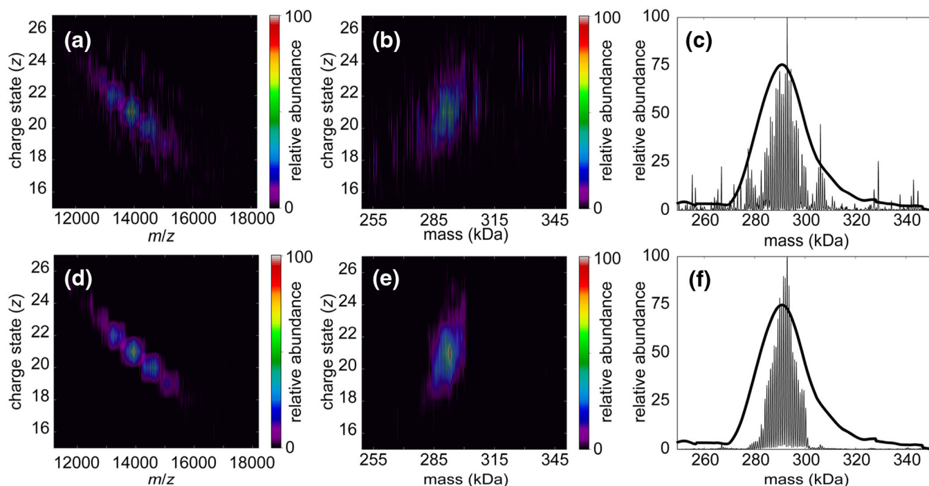
Figure 7. Deconvolved QTOF mass spectra vs. charge (left), mass vs. charge (center), and zero-charge mass spectra (right) of DPPC-MSP1E3D1 Nanodiscs determined using UniDec. Mass spectral data are the same as in Figure 2. (a), (b), and (c) result from using “naive” input parameters for subunit mass, charge state range, peak width, and total mass range, whereas (d), (e), and (f) result from using values obtained from the FT-based method (see text). Smooth black trace in (c) and (f) represents zero-charge mass spectrum reconstructed using FT approach (see Figure 5D)
