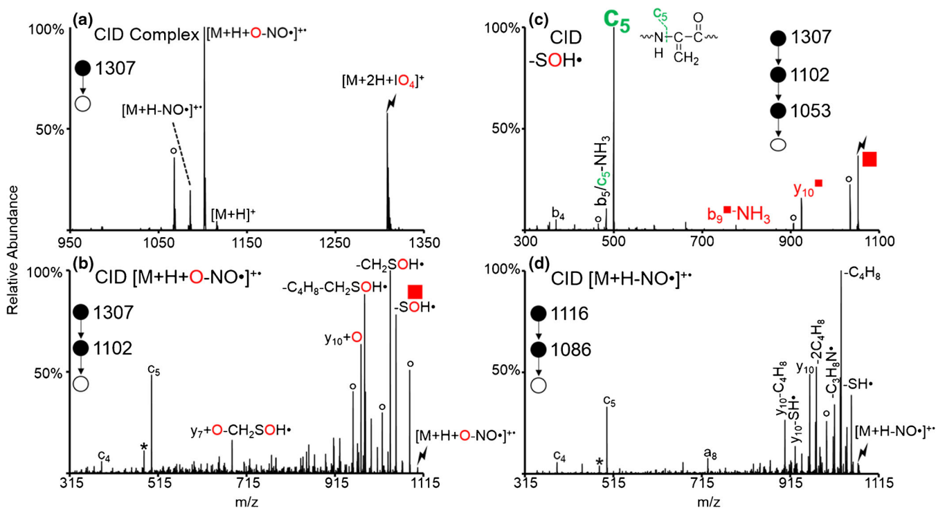
Figure 3. Oxidation of S-NO KGAILCGIALK via ion/ion reactions with \text{IO}_4^- . Ion trap CID of (a) the ion/ion complex between doubly protonated S-NO KGAILCGIALK and \text{IO}_4^- , (b) the oxidized [\text{M}+\text{H}+\text{O}-\text{NO}]^{2+} species, (c) the \text{SOH}\cdot loss species (■) from (b) to generate the Dha species, and (d) the \text{NO}\cdot loss from the protonated peptide (control spectrum). Lightning bolts indicate species subjected to CID, degree signs indicate water losses, and asterisks indicate ammonia losses
