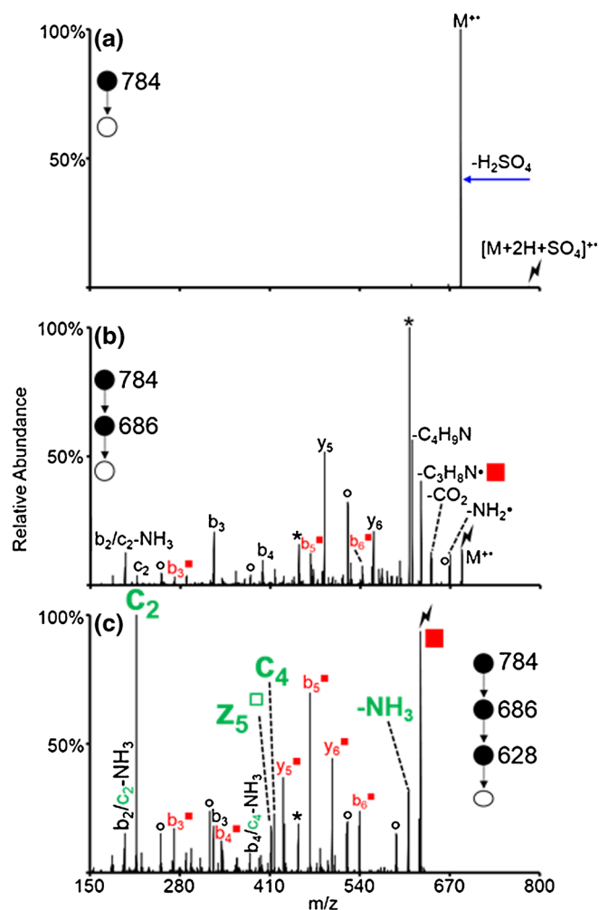
Figure 7. Generation of a molecular radical cation of KAKAKAA via ion/ion reactions with sulfate radical anion. CID of (a) the ion/ion complex between doubly protonated KAKAKAA and \text{SO}_4^{\cdot-} , (b) the molecular radical cation of KAKAKAA, and (c) the loss of \text{C}_3\text{H}_8\text{N}^\bullet from (b) to generate a Dha residue out of one of the lysine residues. Lightning bolts indicate species subjected to CID, asterisks indicate loss of ammonia, degree signs indicate loss of water, red squares indicate Dha-containing species, and fragments derived from the dehydroalanine effect are indicated in green
