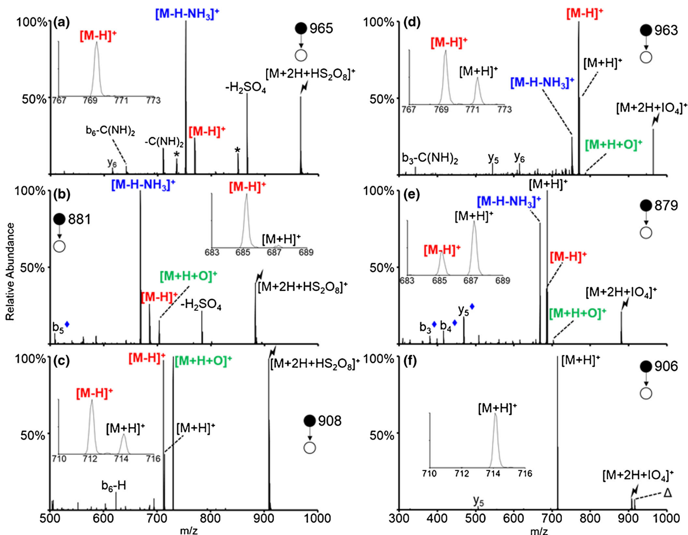
Figure 6. Comparison of the oxidation of neutral basic sites via ion/ion reactions with \text{HS}_2\text{O}_8^- (left) and \text{IO}_4^- (right). CID of the ion/ion complex between doubly protonated RARARAA and (a) \text{HS}_2\text{O}_8^- , (d) \text{IO}_4^- , KAKAKAA and (b) \text{HS}_2\text{O}_8^- , (e) \text{IO}_4^- , and HAHAHAA and (c) \text{HS}_2\text{O}_8^- , (f) \text{IO}_4^- . Lightning bolts indicate species subjected to CID, asterisks indicate loss of ammonia, delta signs indicate contaminants present in the isolation, and blue diamonds indicate [\text{b}/\text{y} - \text{H} - \text{NH}_3]^+ fragments. Insets show the zoomed in mass region around the [\text{M}-\text{H}]^+ and [\text{M}+\text{H}]^+ species
