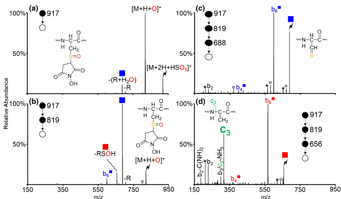
Figure 1. Oxidation of ARAC m AKA via ion/ion reactions with HSO 5 - , where C m indicates a cysteine residue protected with N -hydroxymaleimide. CID of (a) the ion/ion complex between doubly protonated ARAC m AKA and HSO 5 - , (b) the [M+H+O]^+ species, (c) loss of (R + H 2 O) from the oxidized species, and (d) the dehydroalanine species generated upon loss of the alkyl sulfenic acid from the oxidized species. Lightning bolts indicate the species subjected to CID. Asterisks indicate ammonia losses, degree signs indicate water losses, red and blue squares indicate loss of RSOH and (R + H 2 O) from the oxidized species, respectively. Red/blue fragments with square superscripts indicate fragment ions that have lost RSOH/(R + H 2 O)
