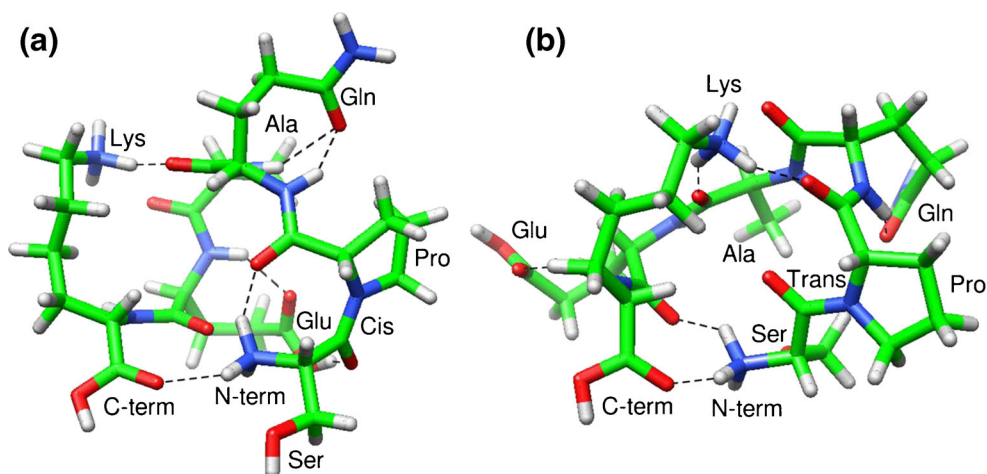
Figure 7. Representative structures of the [\text{SPQAEK} + 2\text{H}]^{2+} ions with \text{Ser}^1\text{-Pro}^2 peptide bond in the cis (a) and trans (b) forms obtained from molecular modeling simulations. Amino acid side chains, terminal regions, and the geometry of the \text{Ser}^1\text{-Pro}^2 bond are labeled for clarity. H-bonds determined using the recommended relaxed constraints in Chimera are represented as dotted lines [43]
