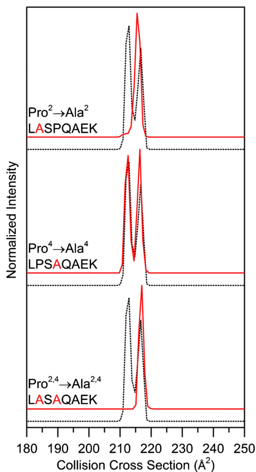
Figure 4. Collision cross section distributions for Pro 2 → Ala, Pro 4 → Ala, and Pro 2,4 → Ala substituted peptides from the [LSPSPQAEK + 2H]^{2+} ions. Substituted distributions are shown in red and the natural sequence is shown as a dotted trace for ease of comparison. Collision cross section distributions for substituted peptides are adjusted for the size difference between Ala and Pro as explained in text
