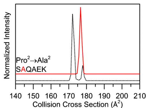
Figure 5. Collision cross section distributions for Pro 2 → Ala from the [SPQAEK + 2H]^{2+} ions. Substituted distributions are shown in red and the natural sequence is shown as a dotted trace for ease of comparison. Collision cross section distributions for substituted peptides are adjusted for the size difference between Ala and Pro as explained in text
