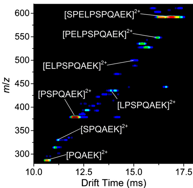
Figure 1. Two-dimensional IMS-MS plot of crude synthesis product of the peptide SPELPSQAEK electrosprayed from 49.5:49.5:1 water:acetonitrile:formic acid. Doubly charged [\text{M} + 2\text{H}]^{2+} truncated sequences of the full-length peptide are labeled
