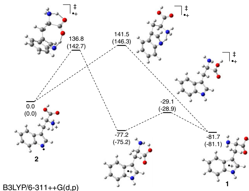
Figure 2. B3LYP/6-311++G(d,p) -calculated reaction pathways for the rearrangement of 2 into 1 . Values reported are \Delta H at 0K and ( \Delta G at 298K)
