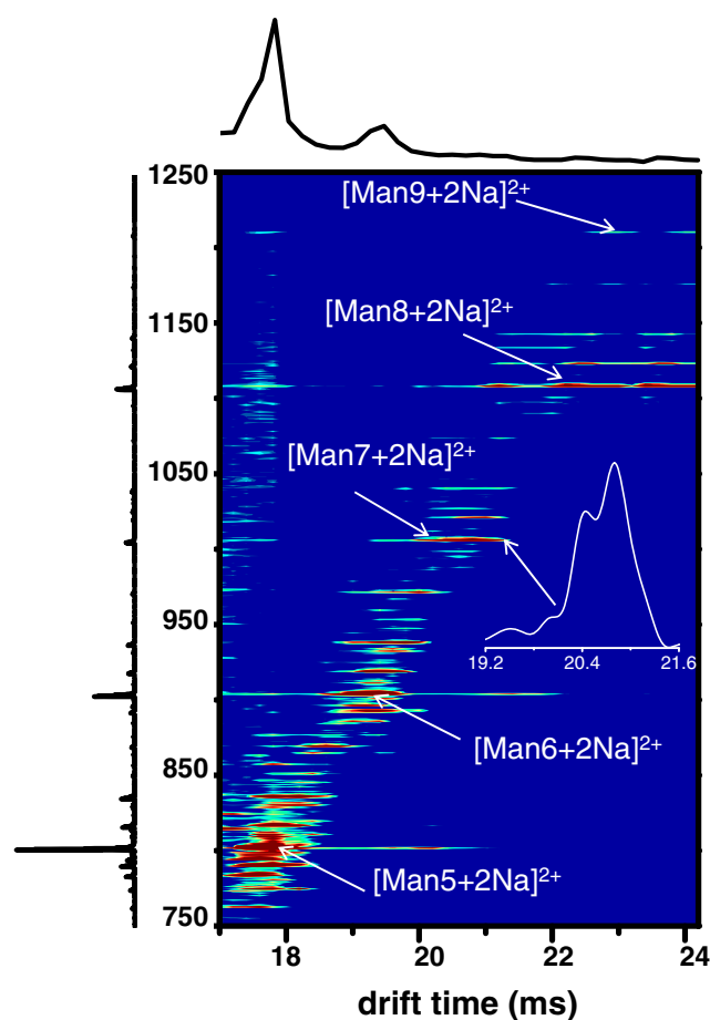
Figure 2. Nested IMS-MS distribution for the electrosprayed high mannose glycans ions derived from RNase B. Across the top is the total drift time distribution obtained by integrating data points over entire m/z range for each drift bin. Across the left shows the total mass spectrum obtained by integrating data points over entire drift range for each m/z bin. Figure inset displays the drift time distribution of the doubly-sodiated \text{Man}_7\text{GlcNAc}_2 glycan ions, obtained by integration of the drift bins across a narrow m/z range
